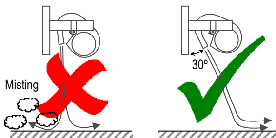
Figure 10: Air Discharge Outlet Angle
