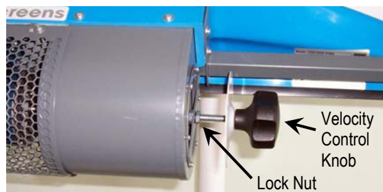
Figure 9: Discharge Air Velocity Control Knob
