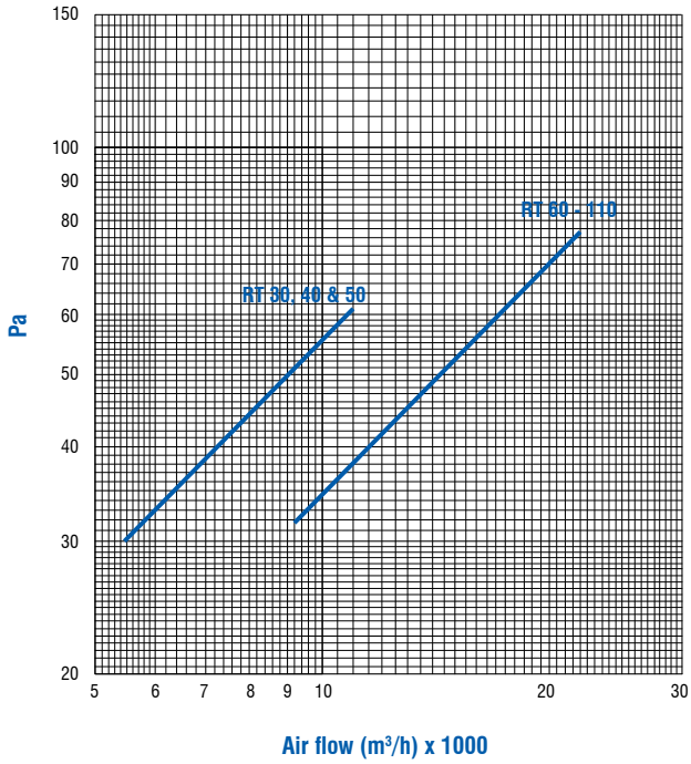
Filter G4
