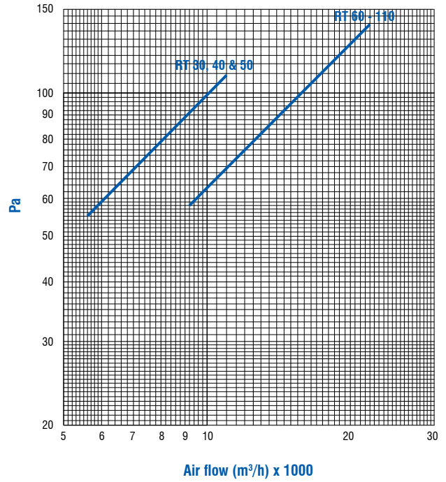
Filter F6
