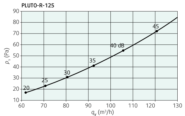
Diagram 1: Pressure drop and A-weighted sound power level
