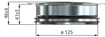
Fig. 1: The PLUTO diffuser dimensions
