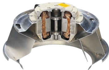
Systemair external rotor motor
