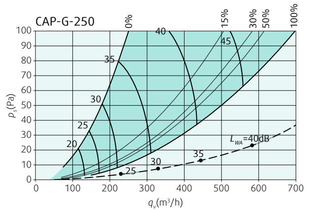
Diagram 4a: Pressure drop and sound power level measured with (continuous lines) and without (dashed line) Thor plenum box.
