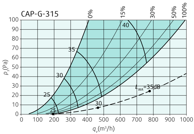
Diagram 5a: Pressure drop and sound power level measured with (continuous lines) and without (dashed line) Thor plenum box.
