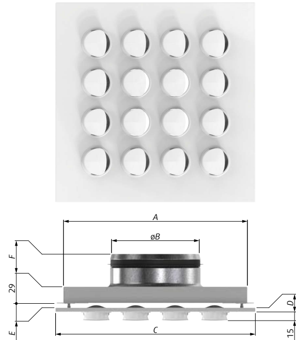
Fig. 1: CAP-G dimensions
