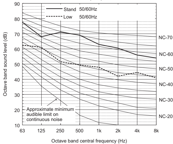
Sound level of PURY-P550YNW-A(-BS)
