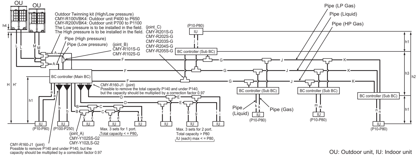
Fig. 12-2-3A Piping scheme
