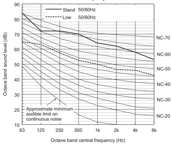
Sound level of PURY-P950YSNW-A(-BS)
