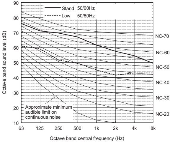
Sound level of PURY-P550YSNW-A(-BS)
