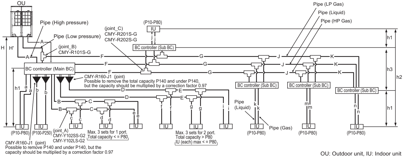
Fig. 12-2-2A Piping scheme
