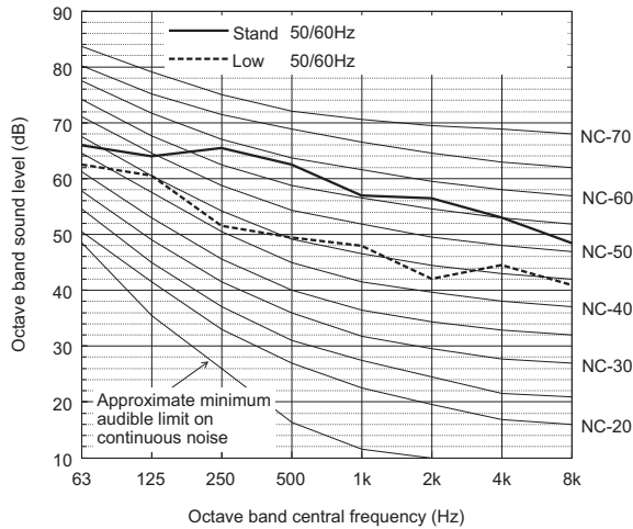
Sound level of PURY-P500YNW-A(-BS)
