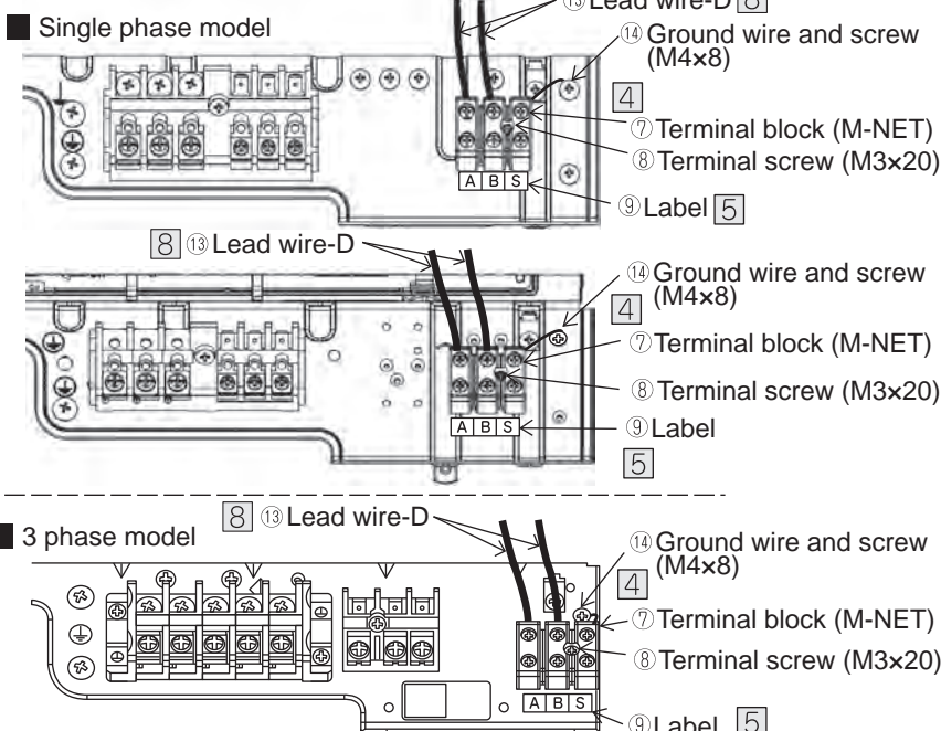
(Viewed from the front of terminal block)
