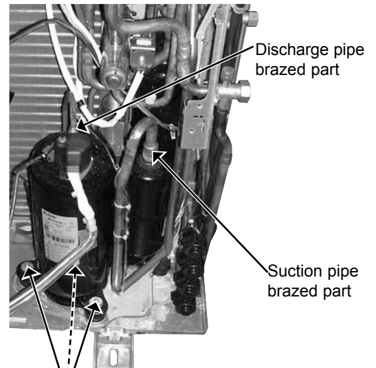
Compressor nuts
