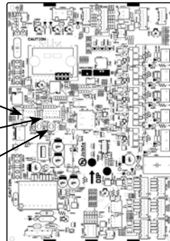
Outdoor control P.C. board
