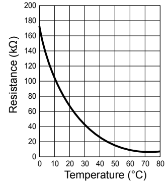
Fin temperature thermistor (RT64)
