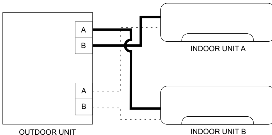
<Incorrect piping>
