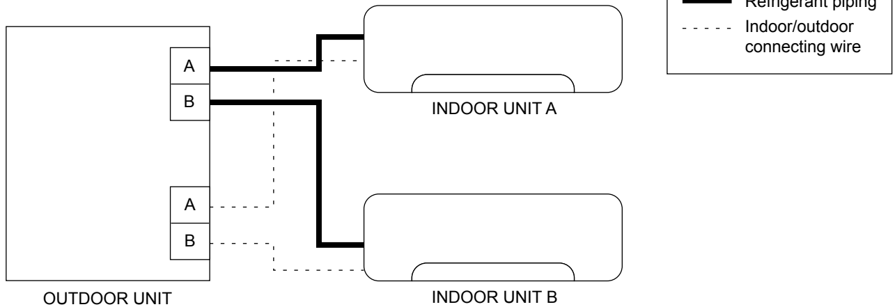
<Correct line>
