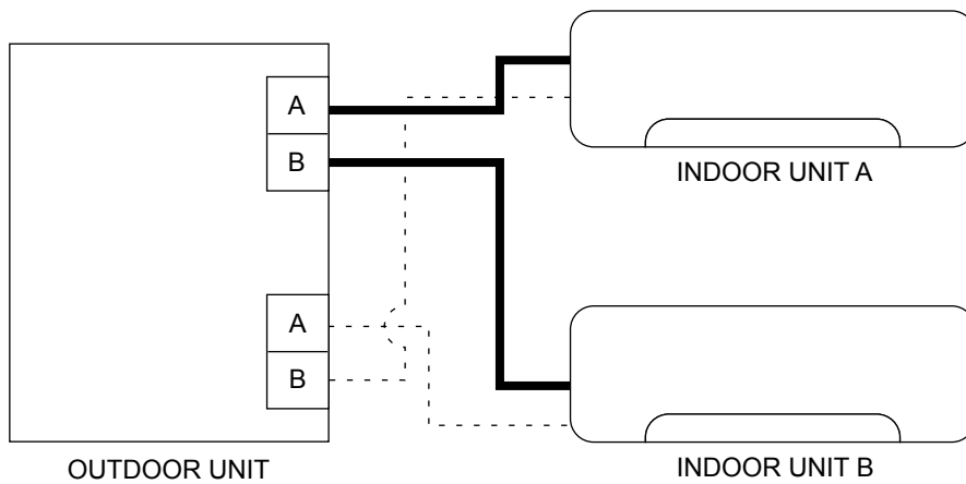
<Incorrect piping>
