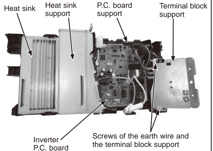
Photo 5 (Inverter assembly)
