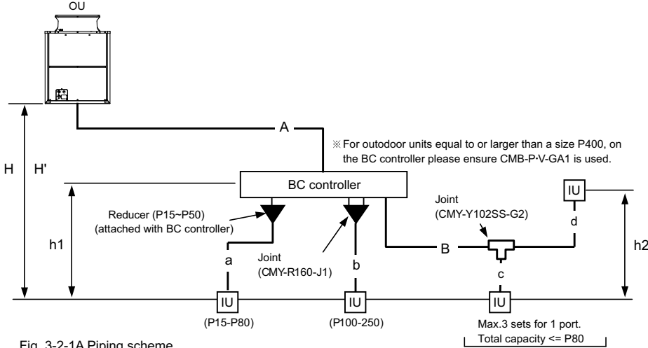
Fig. 3-2-1A Piping scheme
