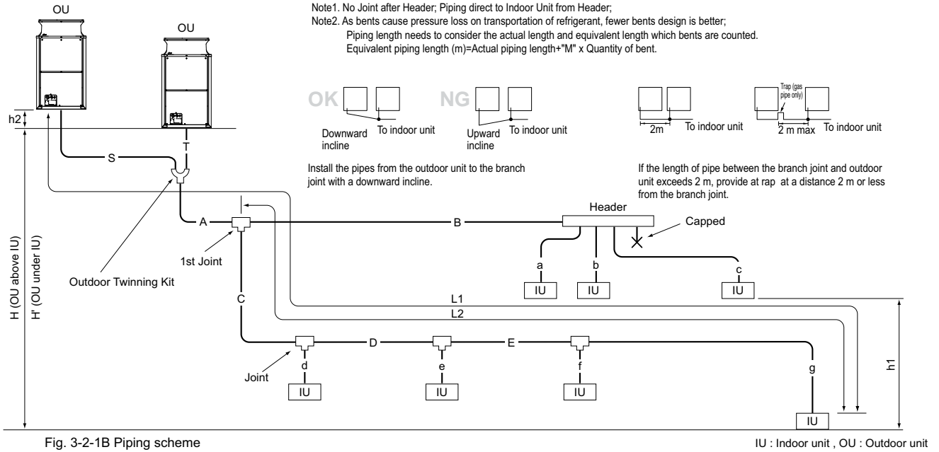
Fig. 3-2-1B Piping scheme
