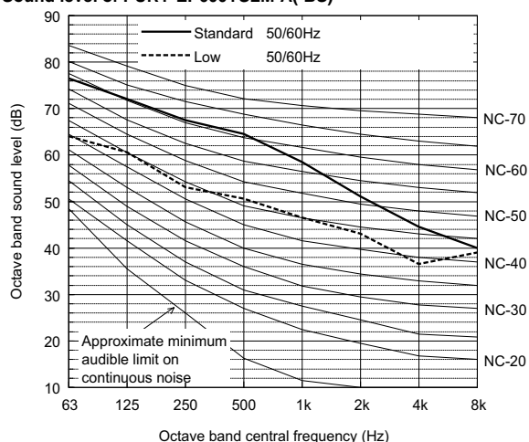
Sound level of PURY-EP600YSLM-A(-BS)
