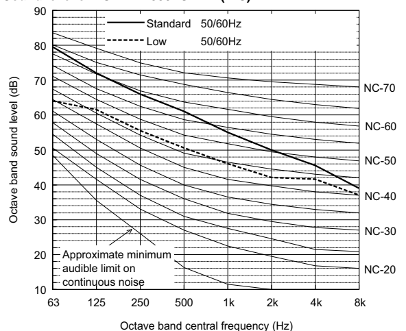
Sound level of PUHY-EP550YSLM-A(-BS)
