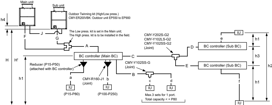
Fig. 3-2-3A Piping scheme
