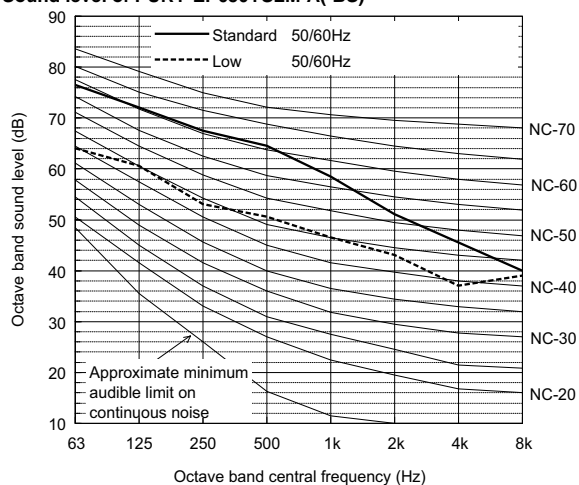
Sound level of PURY-EP650YSLM-A(-BS)
