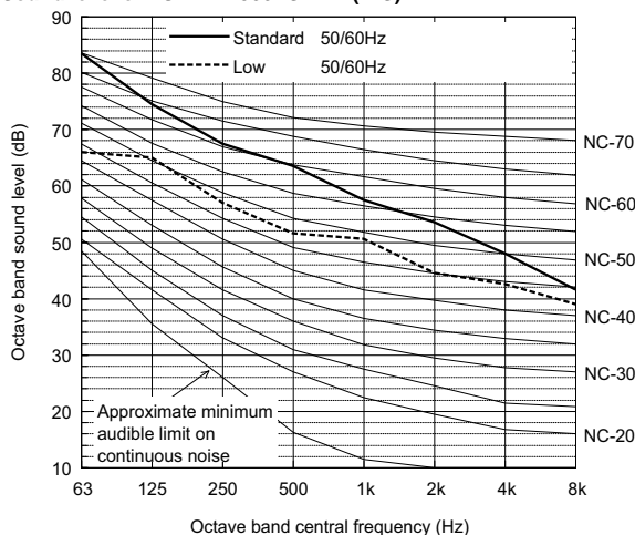
Sound level of PUHY-EP900YSLM-A(-BS)
