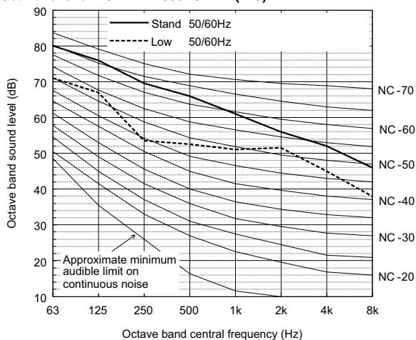
Sound level of PUHY-EP1350YSLM-A(-BS)
