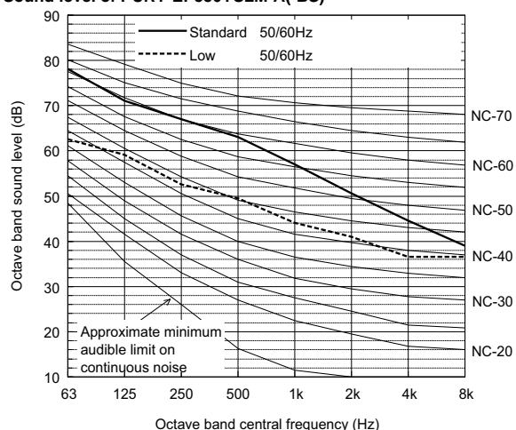
Sound level of PURY-EP550YSLM-A(-BS)
