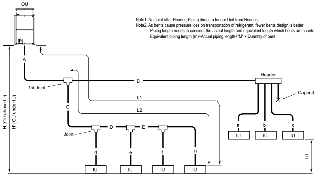
Fig. 3-2-1A Piping scheme
