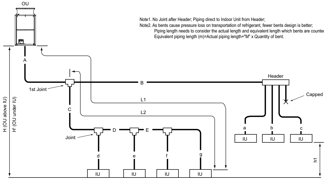
Fig. 3-2-1A Piping scheme
