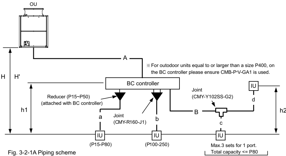
Fig. 3-2-1A Piping scheme
