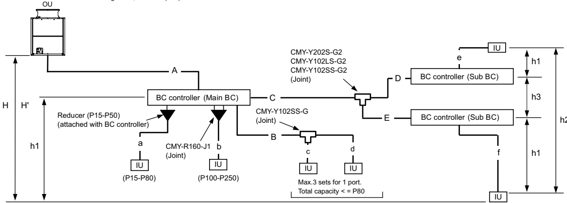
Fig. 3-2-2A Piping scheme
