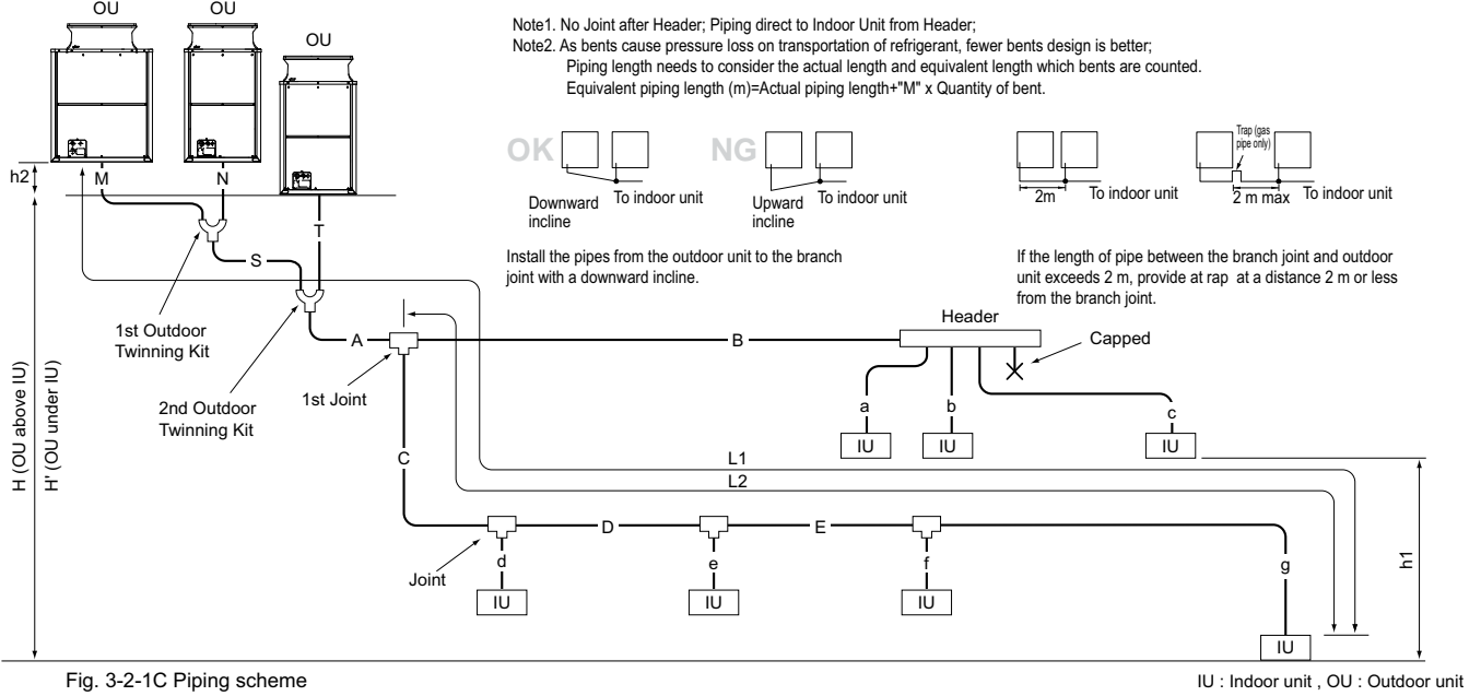
Fig. 3-2-1C Piping scheme
