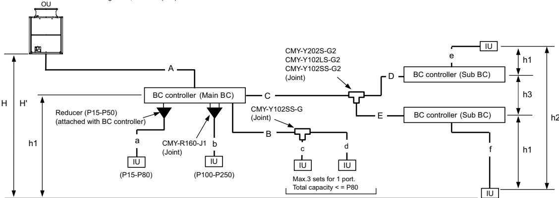
Fig. 3-2-2A Piping scheme
