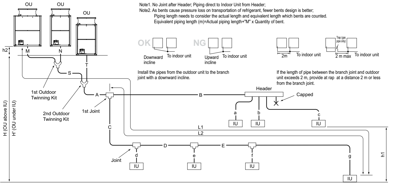
Fig. 3-2-1C Piping scheme
