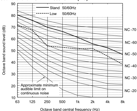
Sound level of PUHY-EP1300YSLM-A(-BS)
