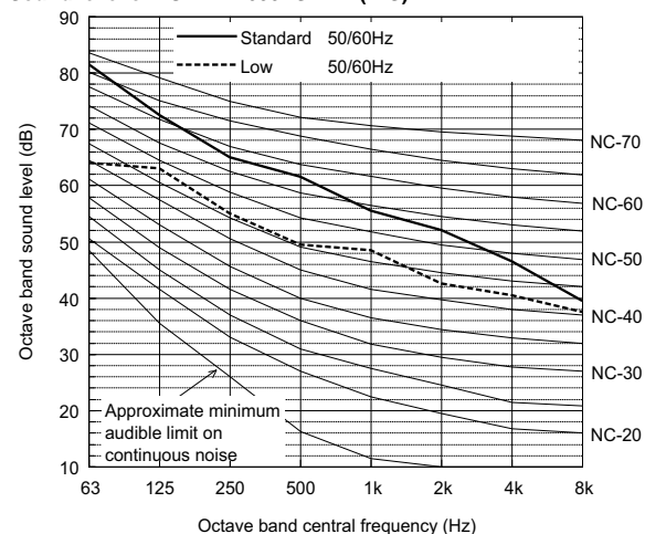
Sound level of PUHY-EP600YSLM-A(-BS)
