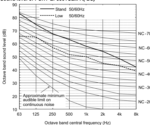
Sound level of PUHY-EP950YSLM-A(-BS)
