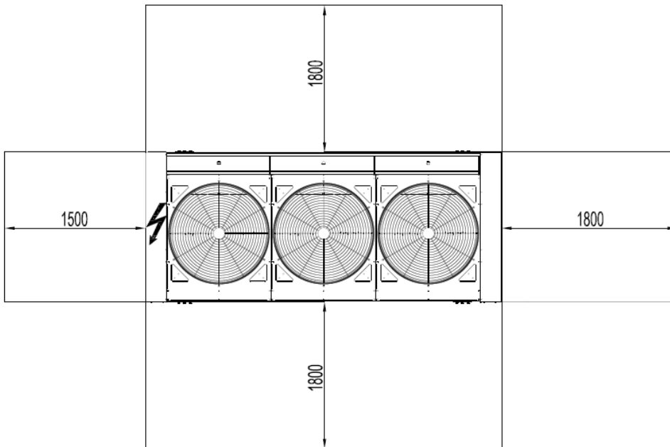
Minimum recommended installation clearances
