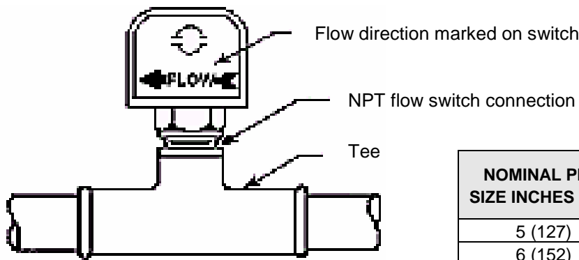
Figure 4 – Flow Switch
