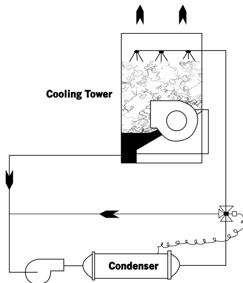
Figure 2, Bypass valve
