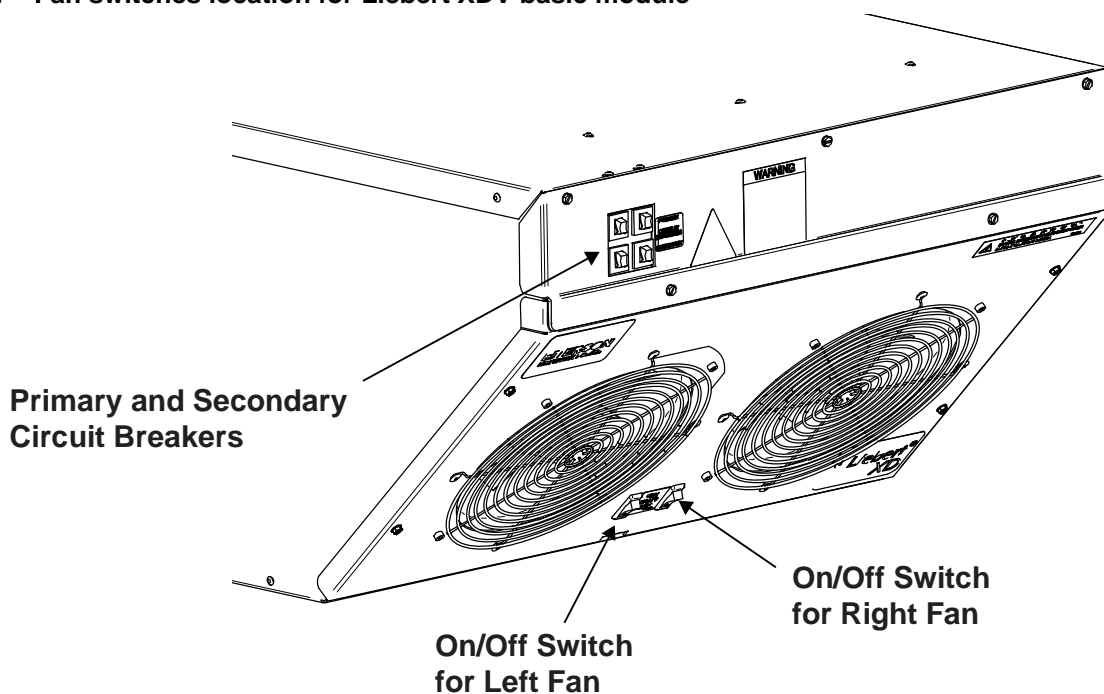
Figure 57 Fan switches location for Liebert XDV basic module
