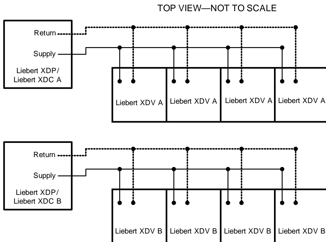
Figure 22 Typical Liebert XDV piping—non-interlaced connection
