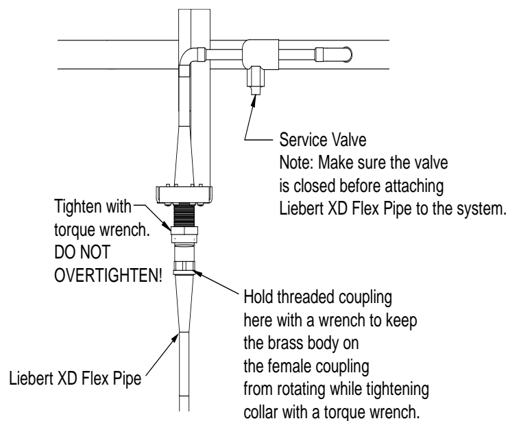
Figure 38 Detail view of Liebert XD Flex Pipe and prefabricated piping port
