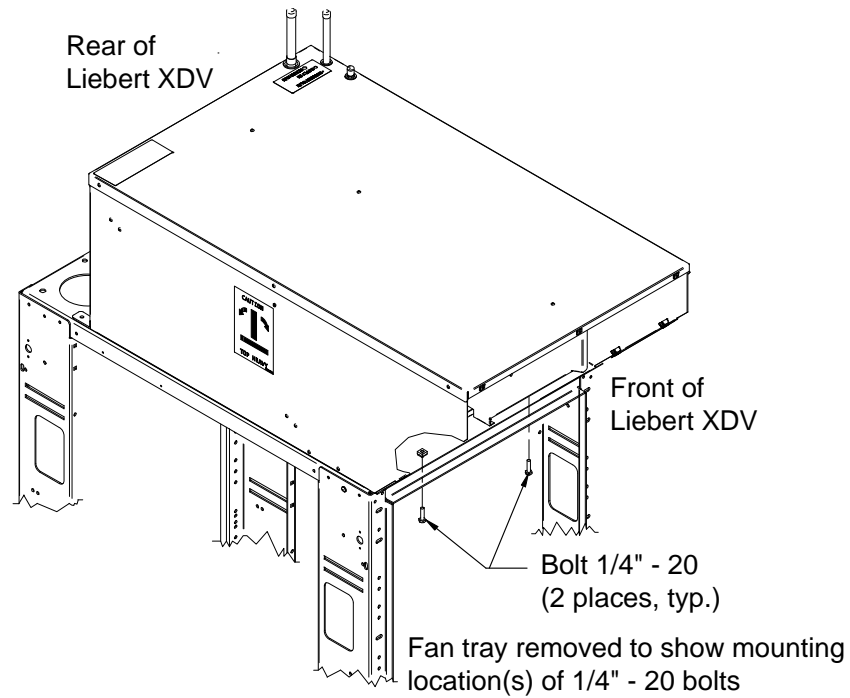
Figure 11 Mounting hole locations—standard mounting method
