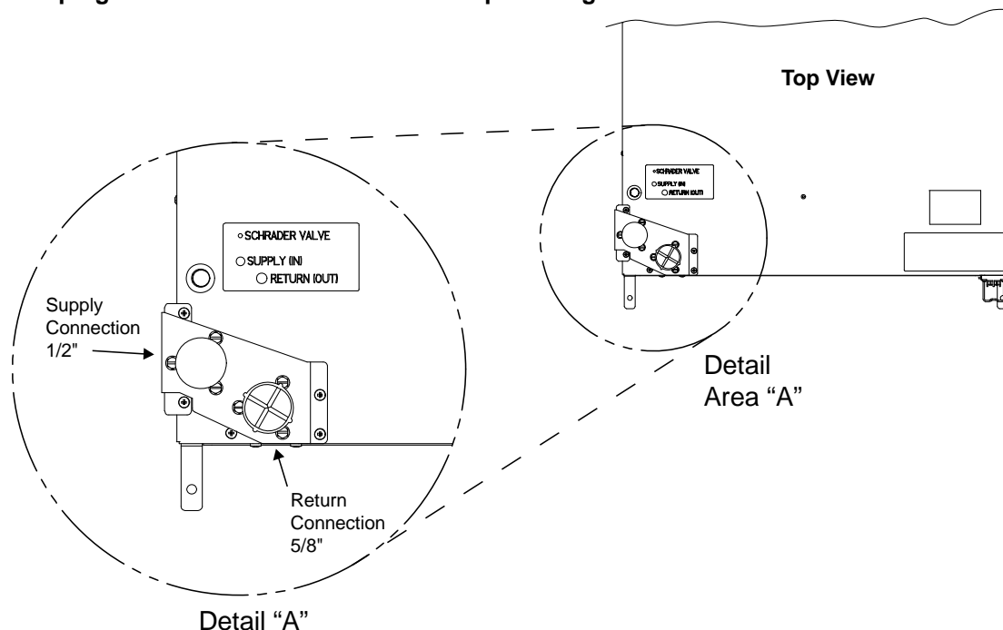
Figure 28 Piping location and connection sizes—pre-charged modules with one-shot connections
