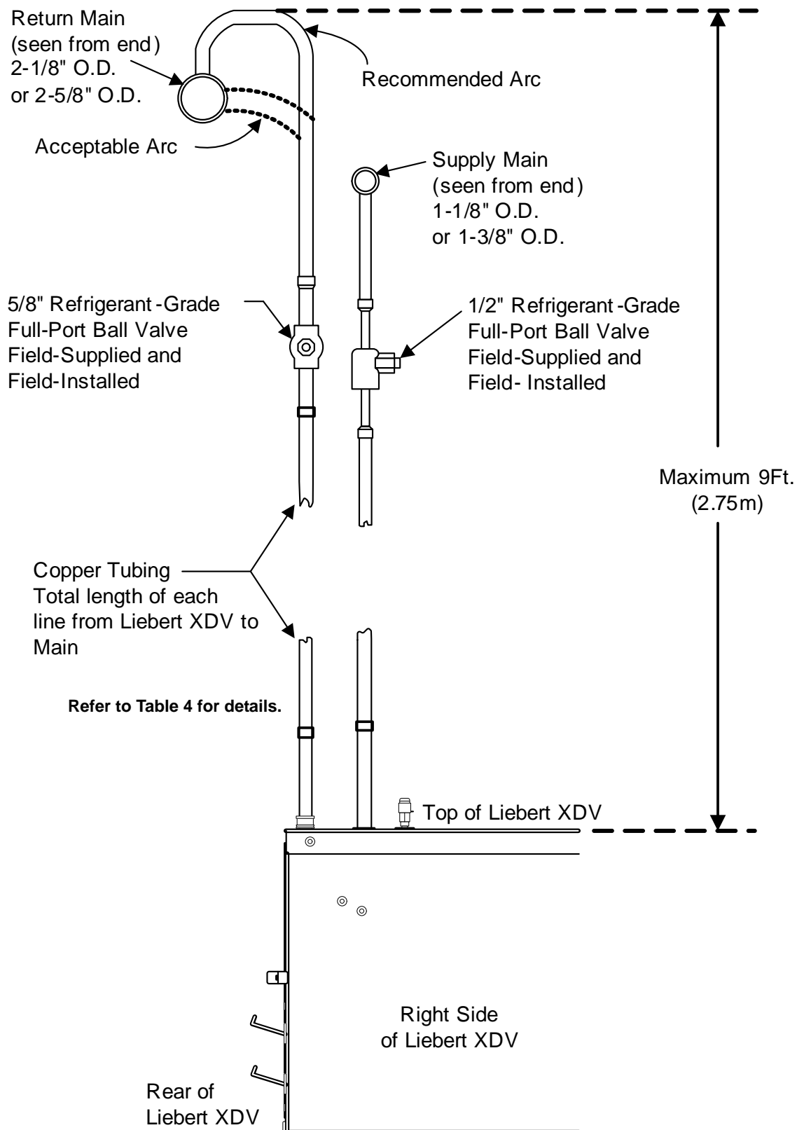
Figure 26 Hard-piped connection diagram
