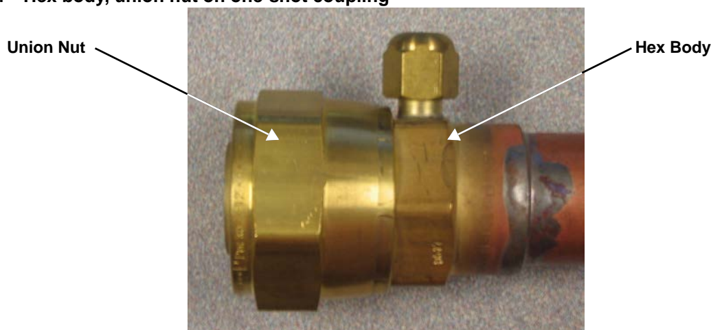
Figure 31 Hex body, union nut on one-shot coupling
