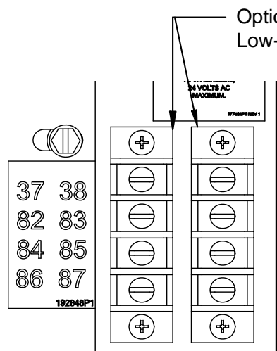
Figure 46 Low-voltage connections for Liebert XDV smart modules
