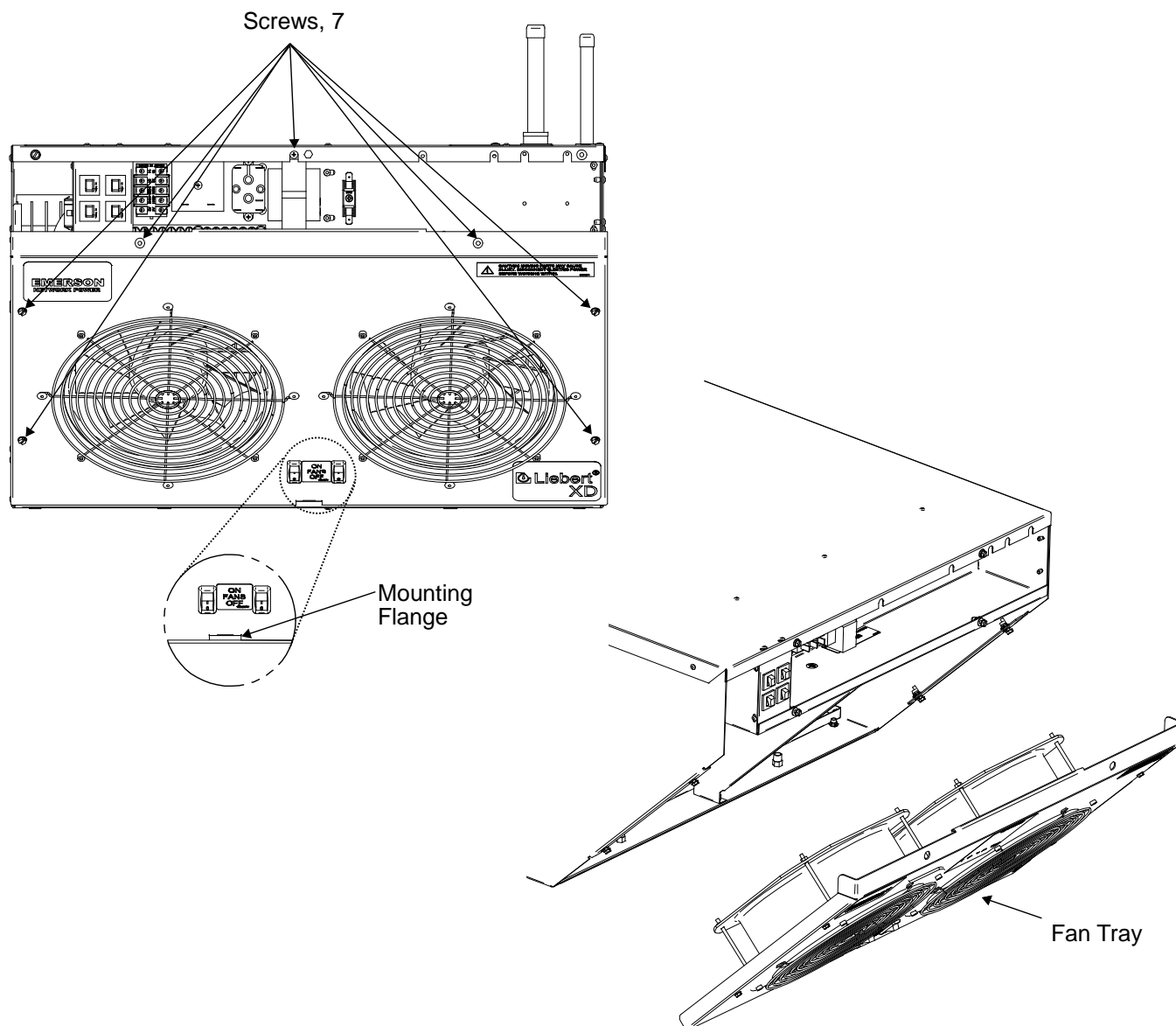
Figure 60 Removing the fan tray
