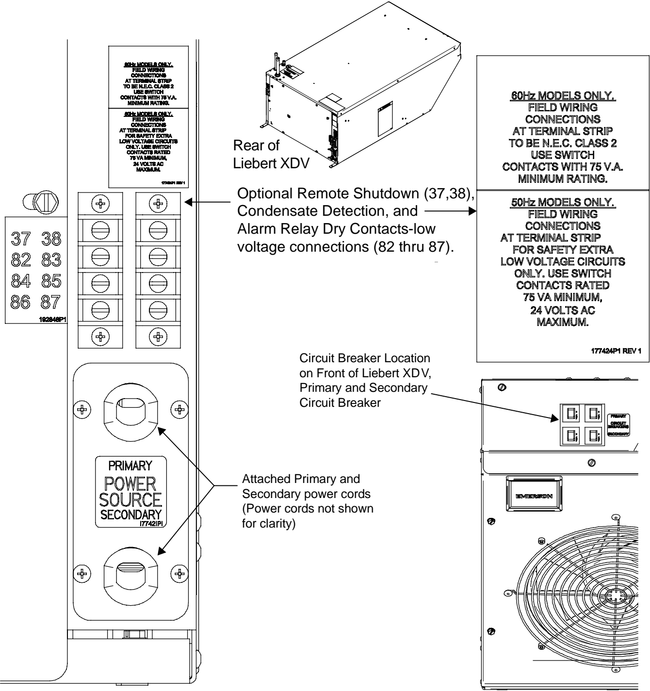
Figure 45 Electrical connections for CE-approved Liebert XDV smart modules
