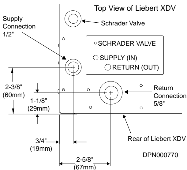
Figure 24 Schrader valve location for venting holding charge
