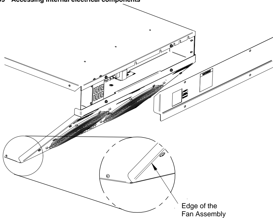
Figure 59 Accessing internal electrical components
