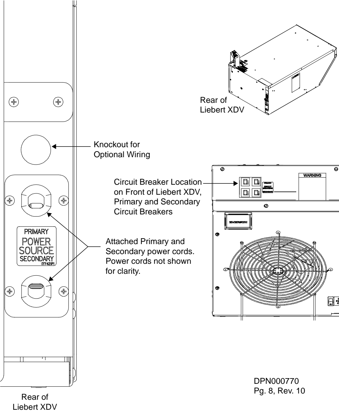
Figure 43 Electrical connections for CE-approved Liebert XDV basic modules
