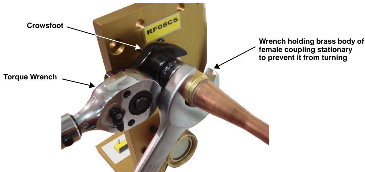
Figure 38 Detail view of Liebert XD Flex Pipe and prefabricated piping port
