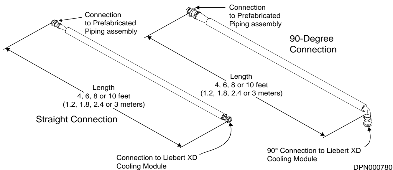
Figure 27 Liebert XD Flex Pipe dimensions—straight and 90-degree connections
