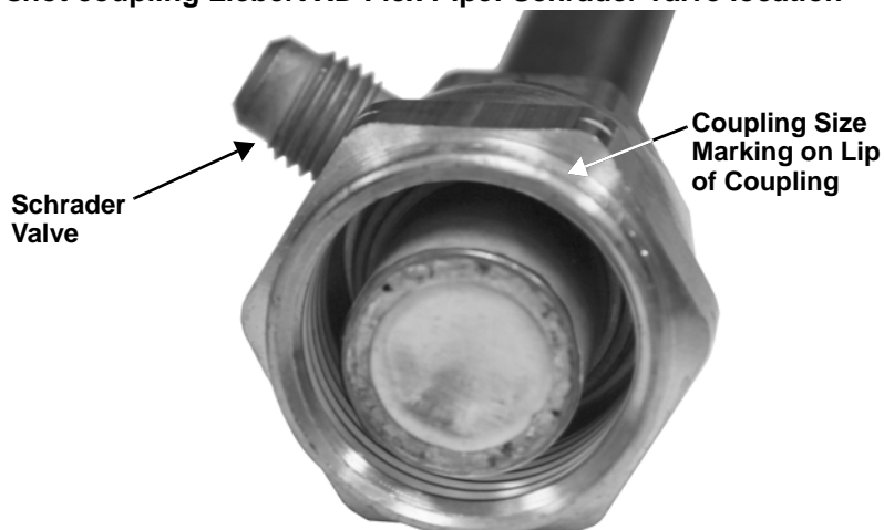
Figure 30 Female one-shot coupling Liebert XD Flex Pipe: Schrader valve location
