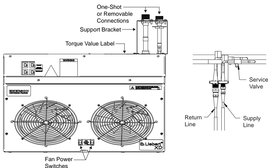
Figure 40 Profile view of the Liebert XD system with Liebert XD Flex Pipe connections
