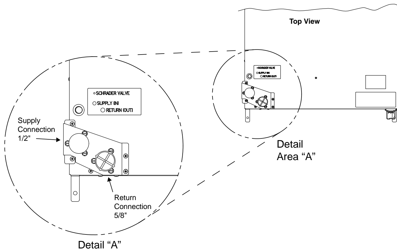
Figure 32 Piping location and connection sizes—removable connections
