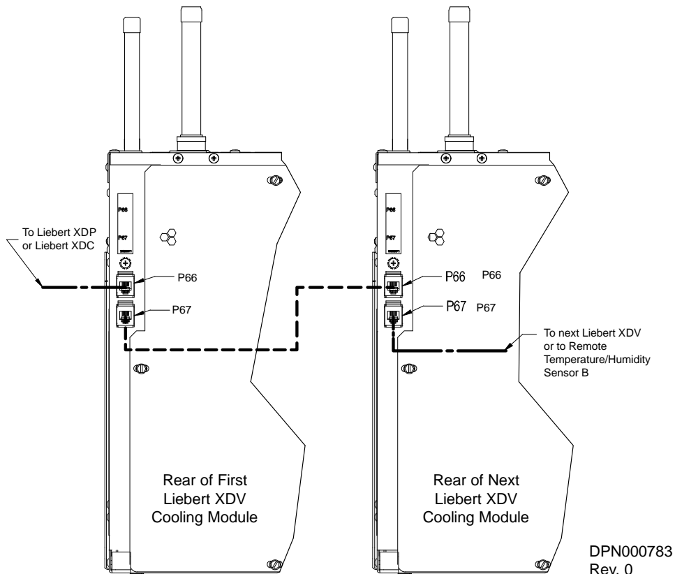
Figure 54 Liebert XDV Smart Module CANbus port locations
