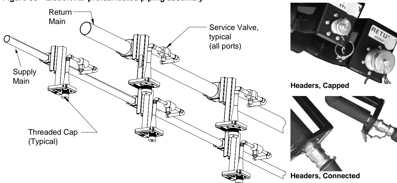
Figure 35 Liebert XD prefabricated piping assembly
