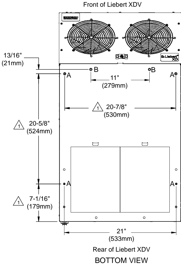
Figure 12 Mounting hole locations—alternate mounting points
