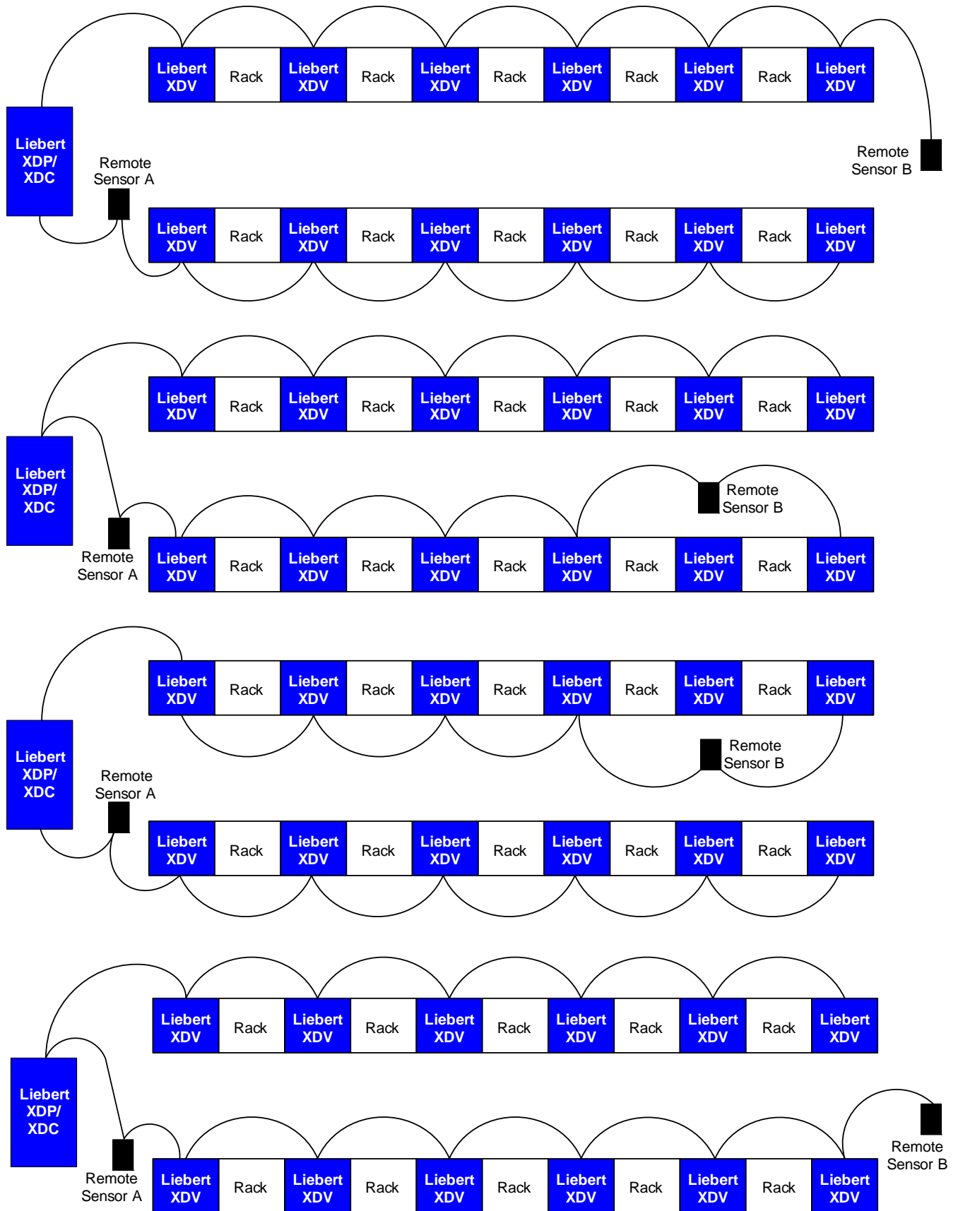
Figure 49 Modules on two chains
