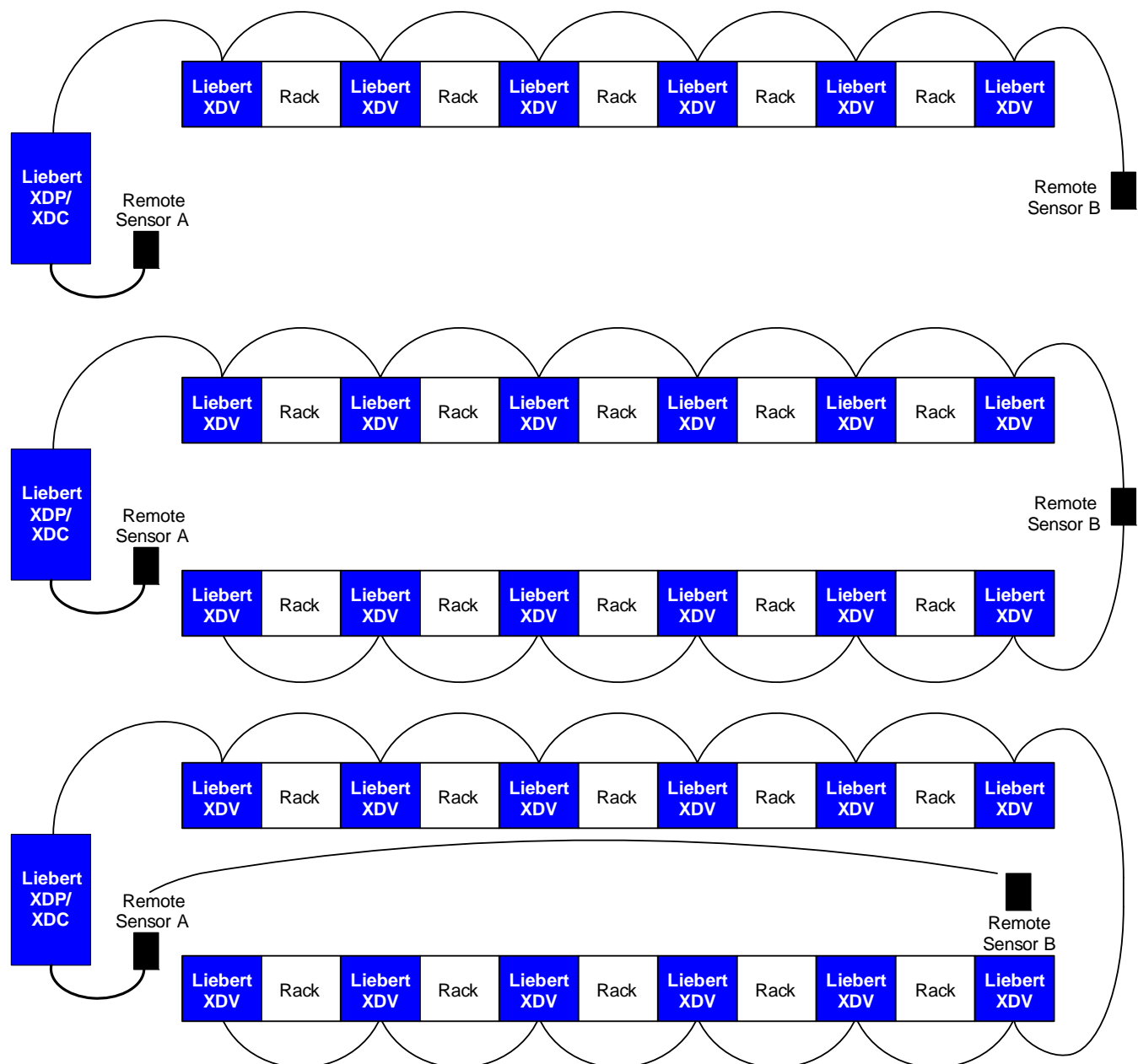
Figure 48 Modules on a single chain
