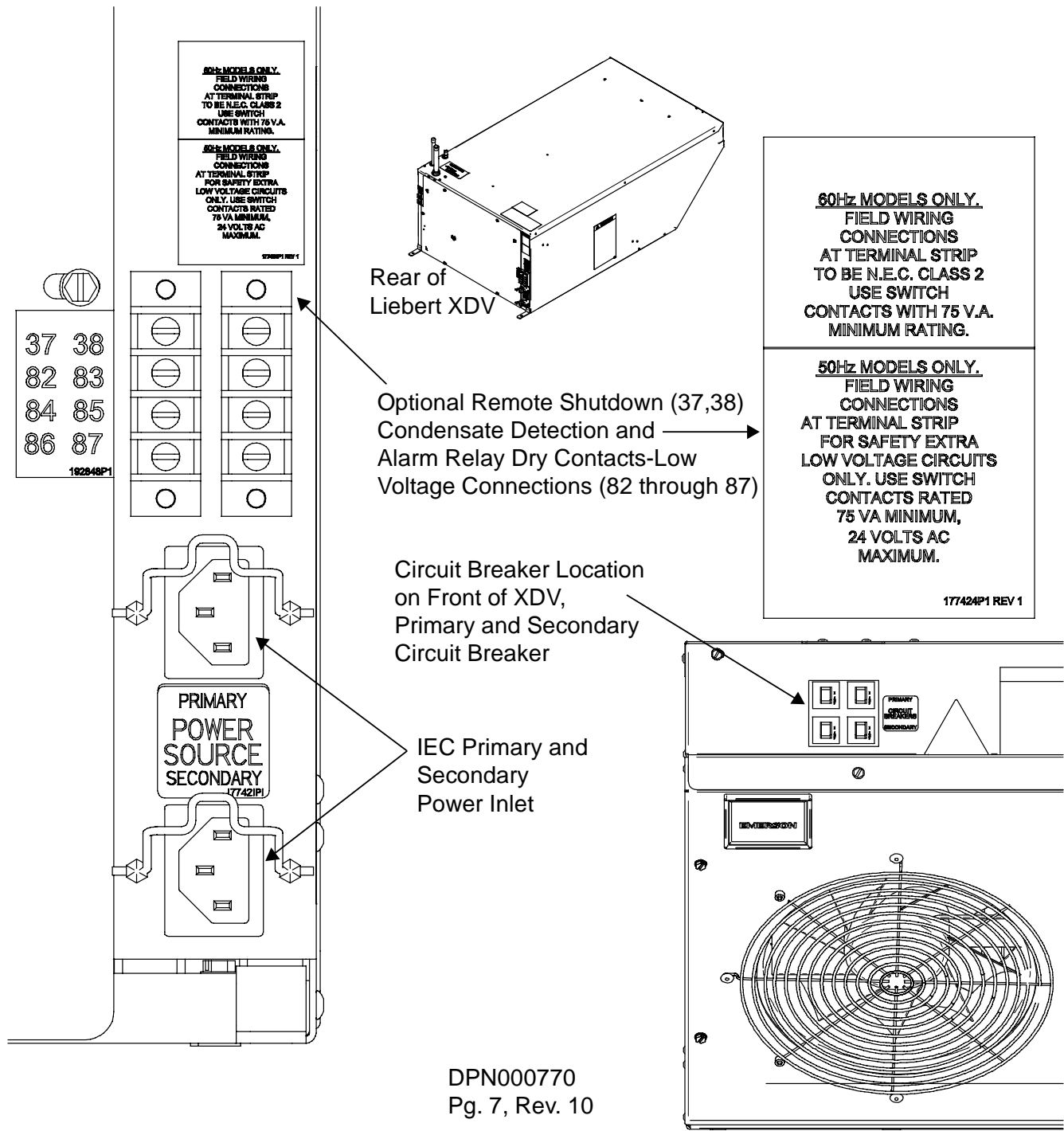
Figure 44 Electrical connections for CSA-approved Liebert XDV smart modules
