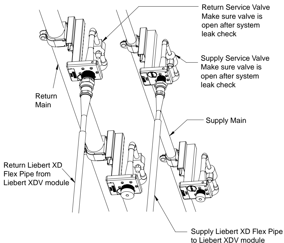
Figure 39 Liebert XD system with prefabricated piping assembly and Liebert XD Flex Pipe
