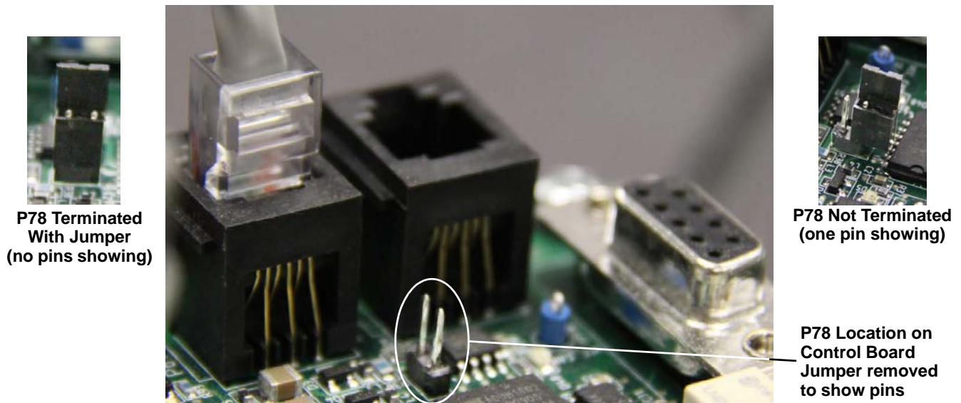
Figure 56 Liebert XD smart module P78 location
