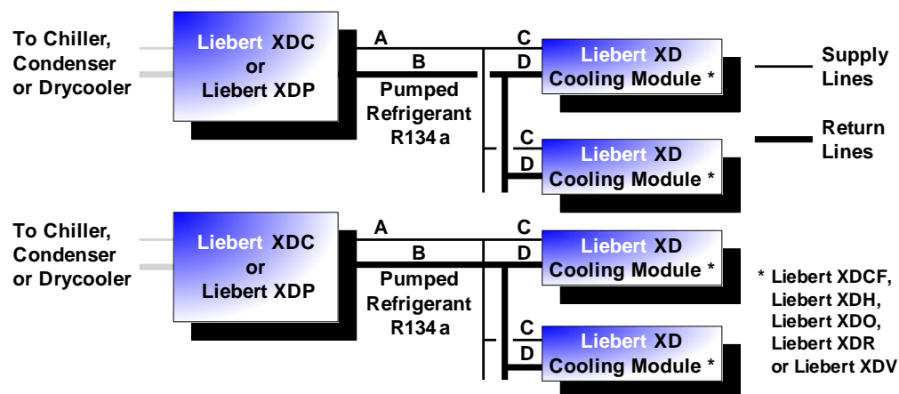
Figure 25 Generic piping layout
