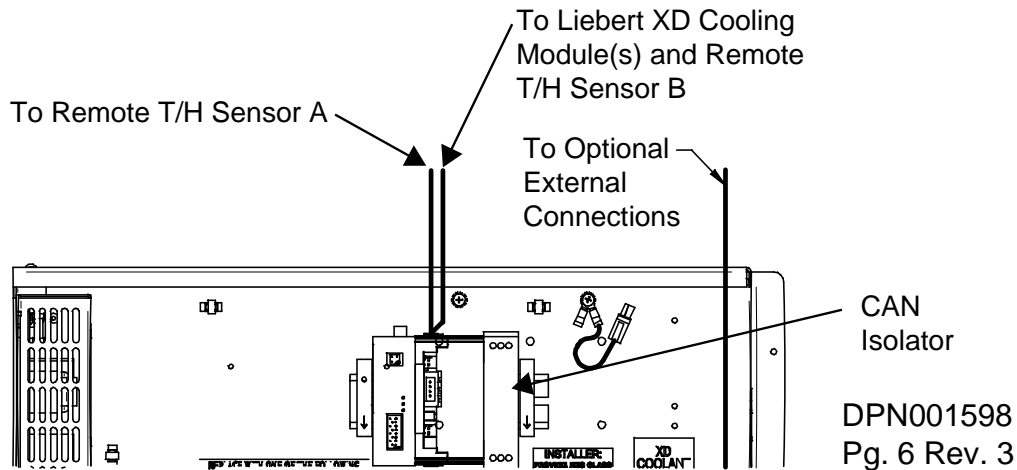
Figure 52 CAN Isolator location within the Liebert XDP/XDC
