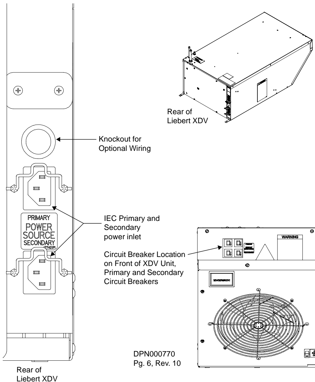
Figure 42 Electrical connections for CSA-approved Liebert XDV basic modules
