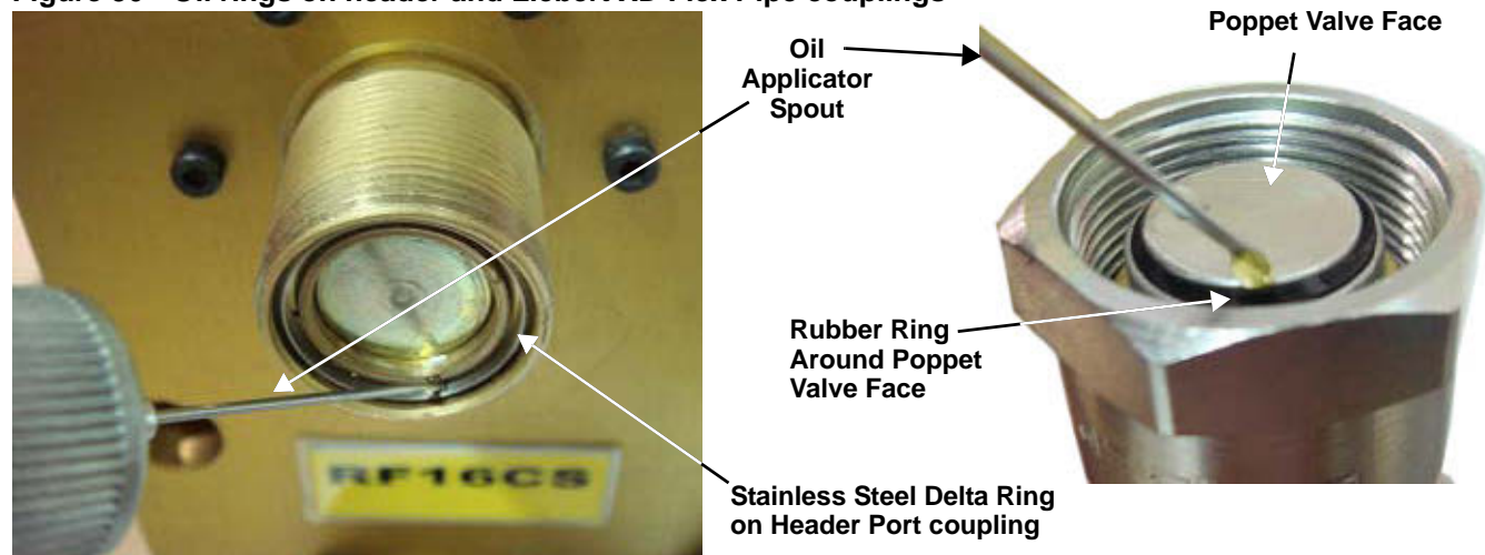
Figure 36 Oil rings on header and Liebert XD Flex Pipe couplings
