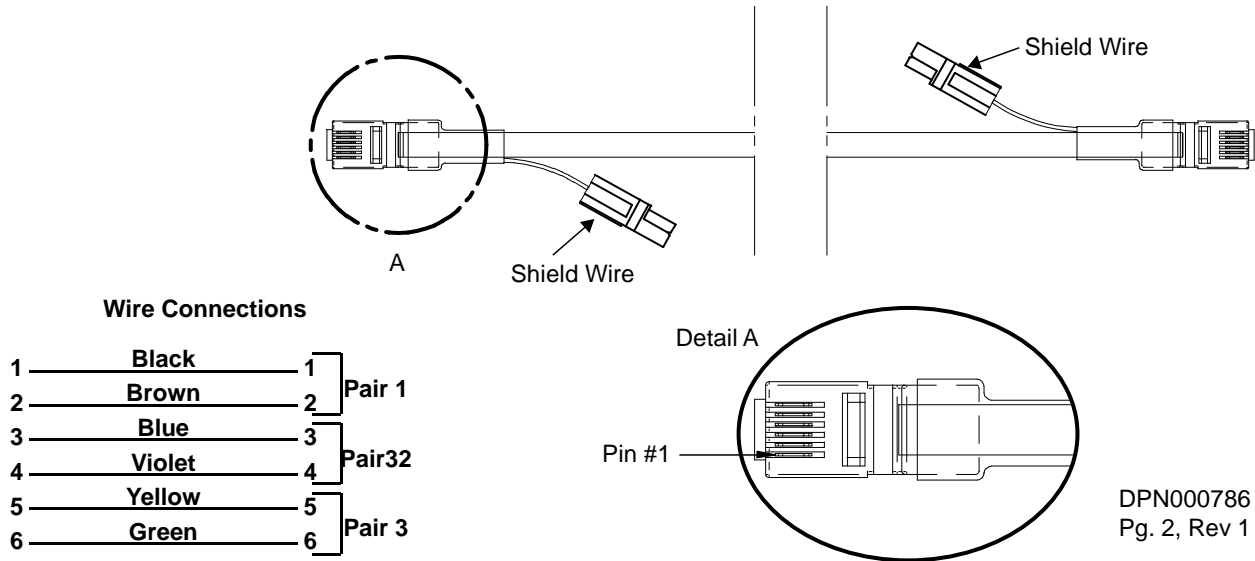
Figure 51 CANbus cable plug
