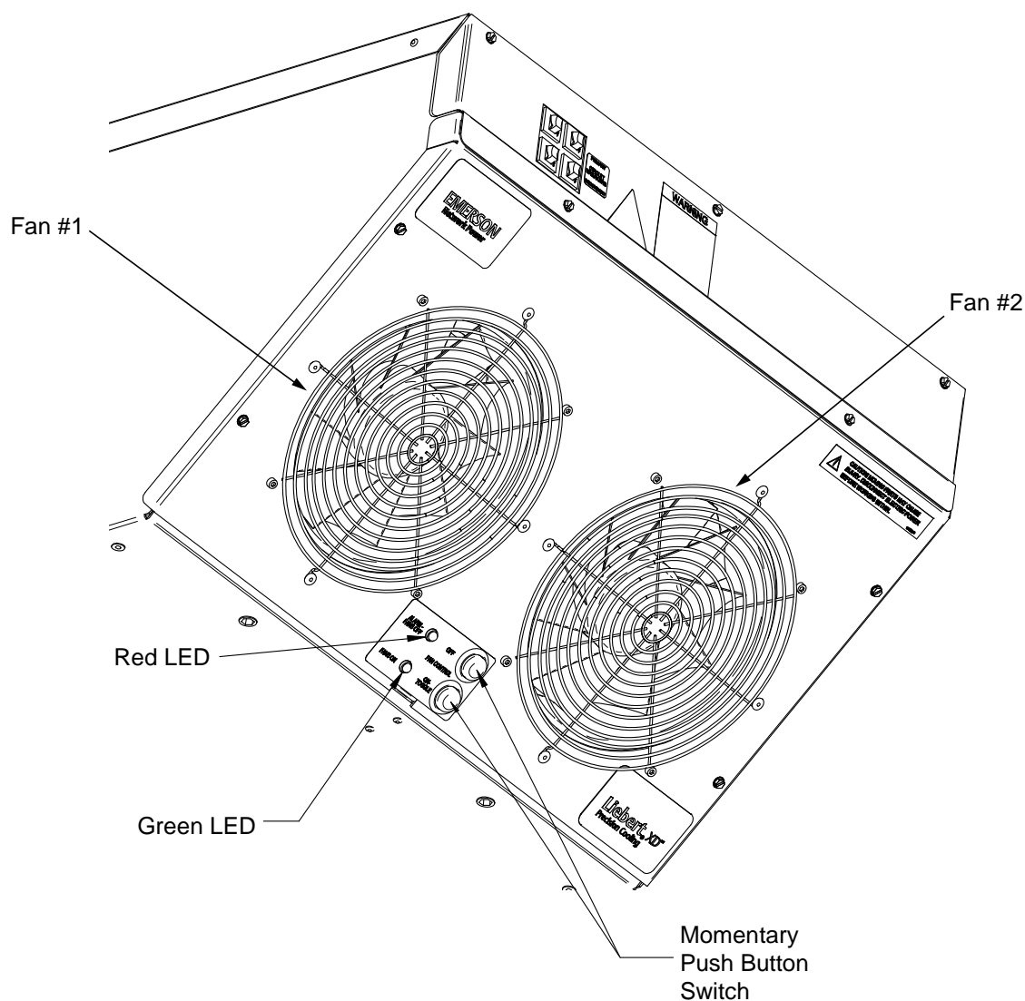
Figure 58 Fan switches with push buttons and LEDs for Liebert XDV smart module
