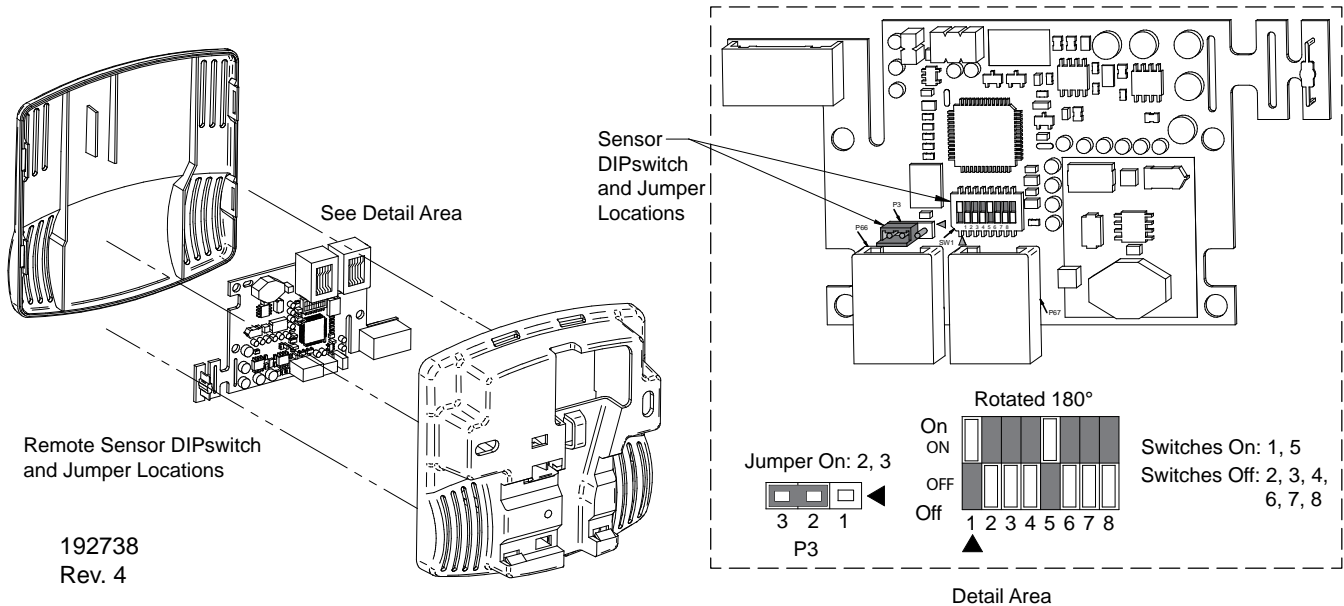
Figure 55 Removing remote sensor cover; temperature and humidity sensor jumper location
