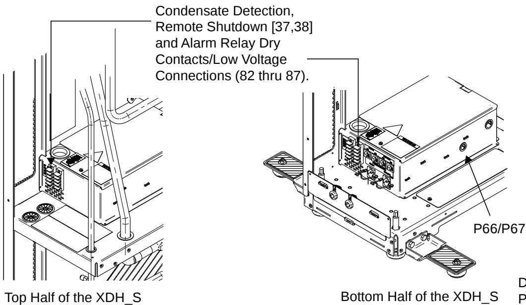
Figure 36 Low-voltage connections—Liebert XDH smart module
