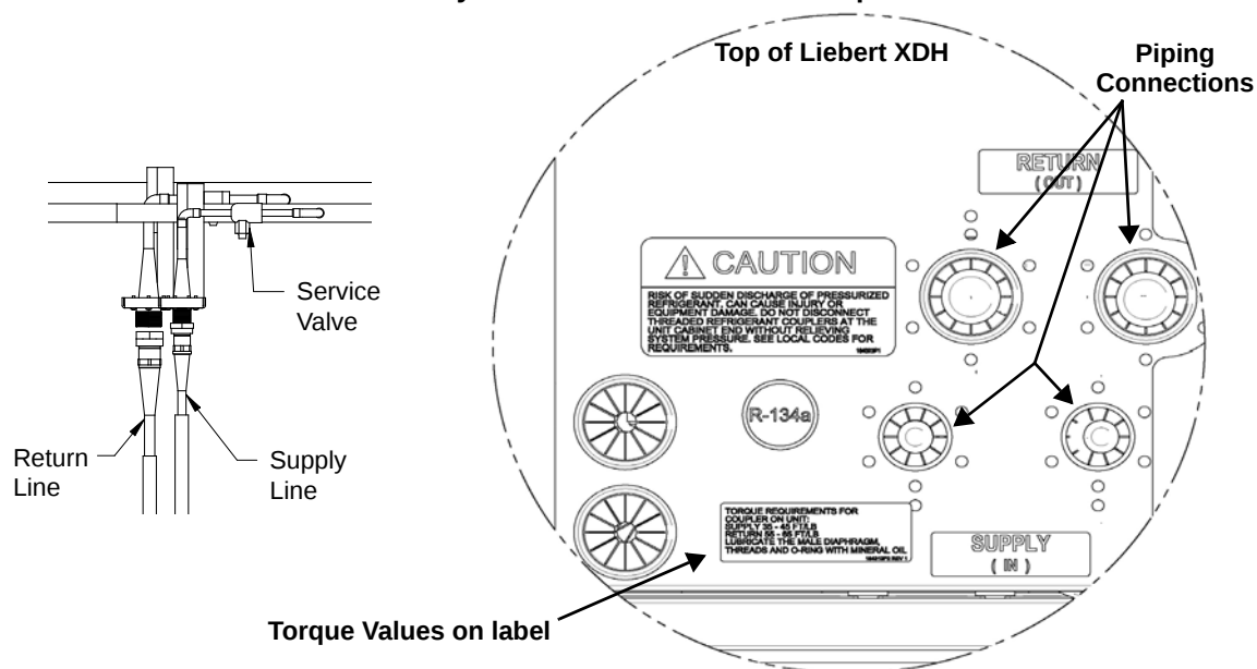
Figure 31 Profile view of the Liebert XD system and Liebert XD Flex Pipe location
