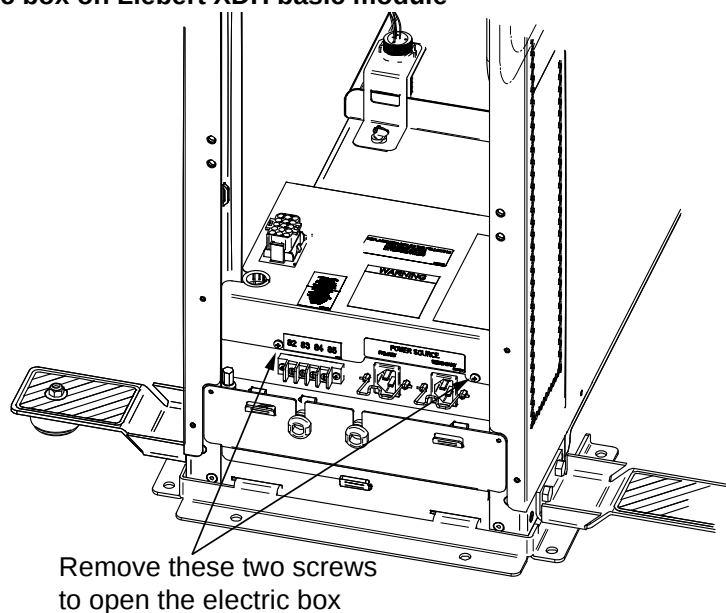
Figure 53 Open electric box on Liebert XDH basic module
