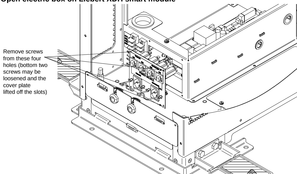
Figure 54 Open electric box on Liebert XDH smart module
