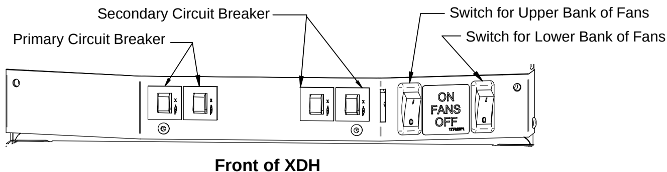
Figure 49 Fan switches, Liebert XDH basic modules
