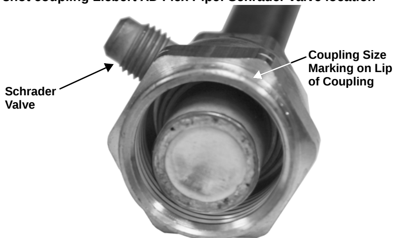
Figure 21 Female one-shot coupling Liebert XD Flex Pipe: Schrader valve location
