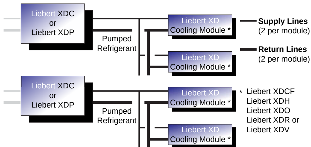
Figure 3 Generic piping layout
