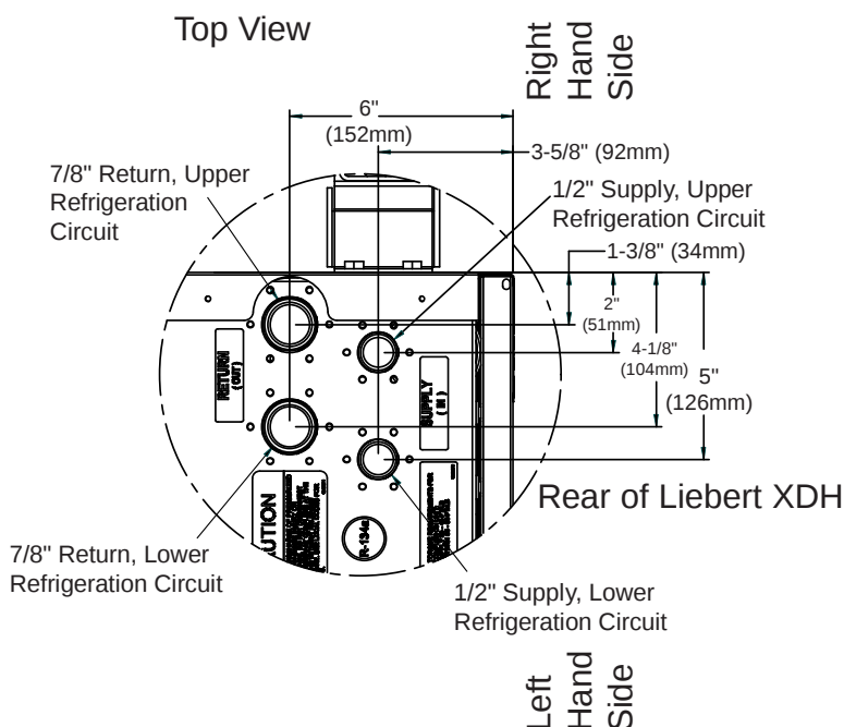
Figure 19 Piping location and connecting sizes for pre-charged modules
