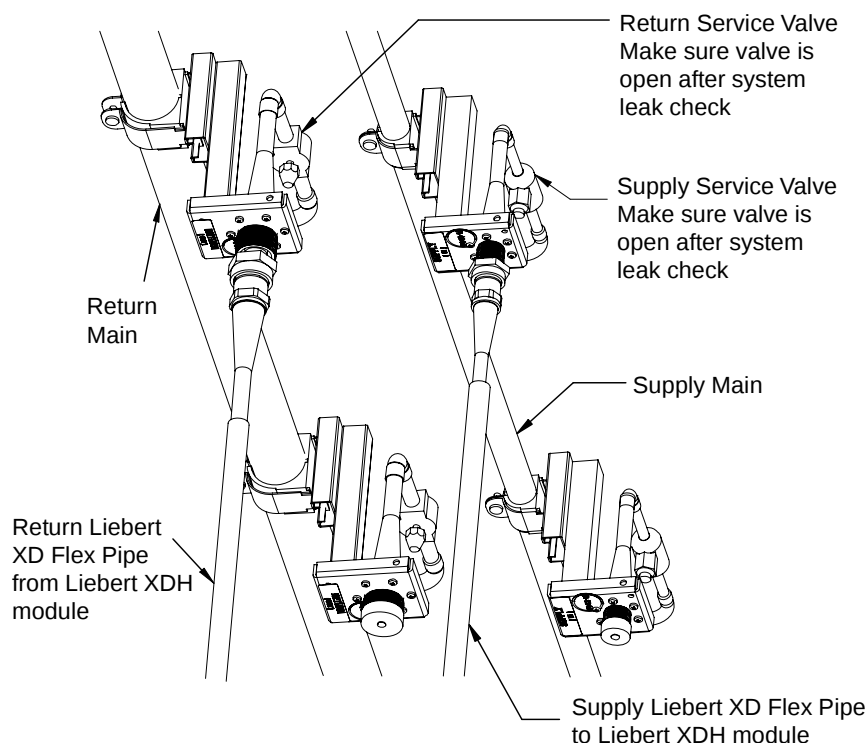
Figure 30 Liebert XD system with prefabricated piping assembly and Liebert XD Flex Pipe
