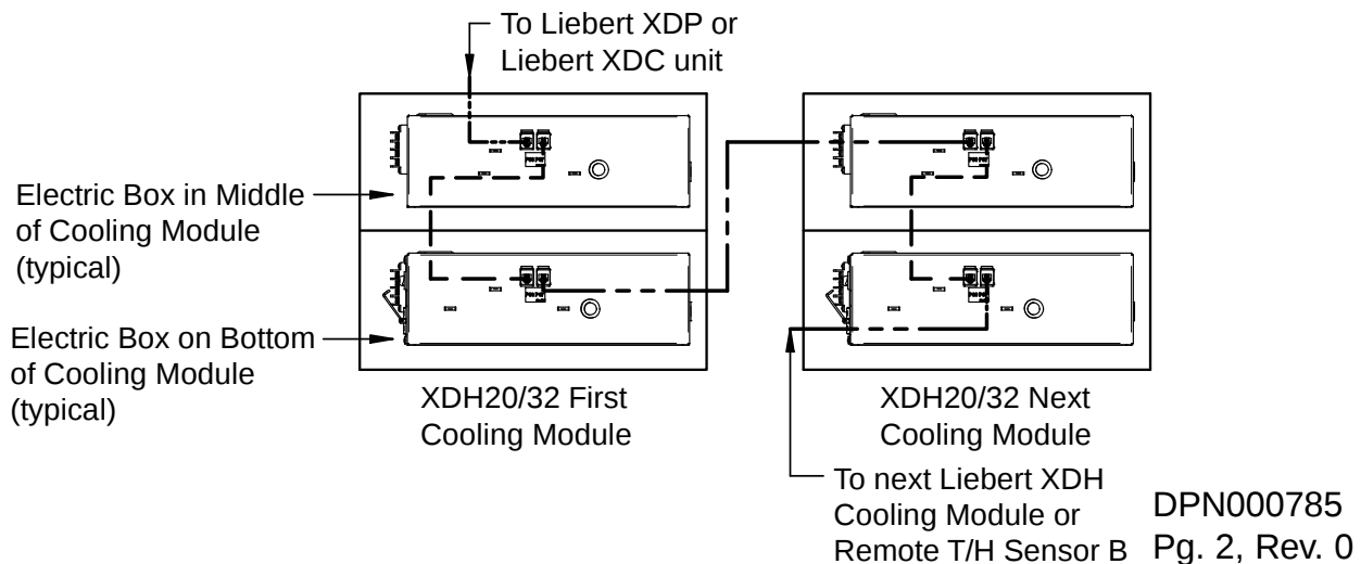
Figure 45 Single-circuited Liebert XDHs
