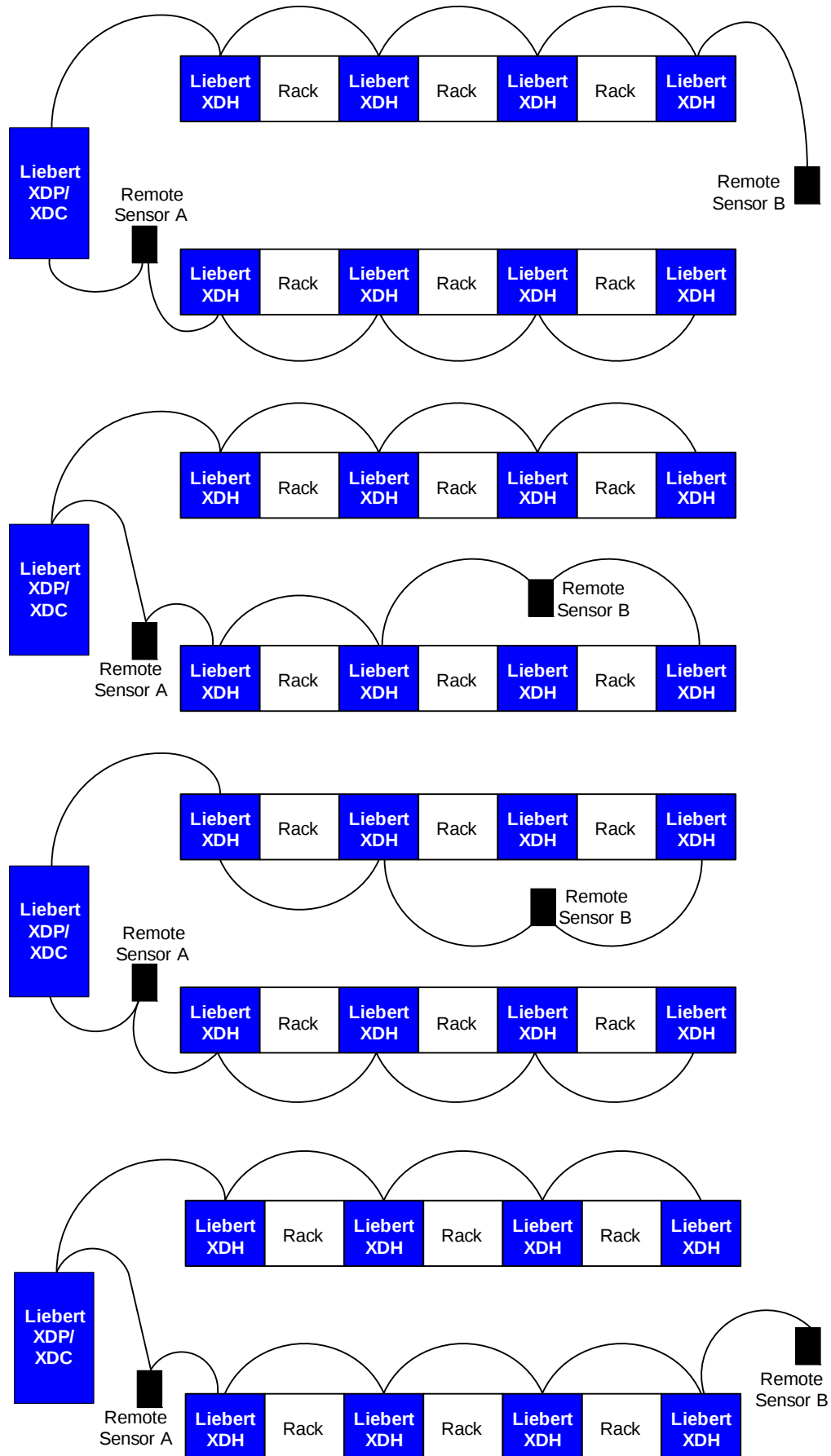
Figure 39 Modules on two chains
