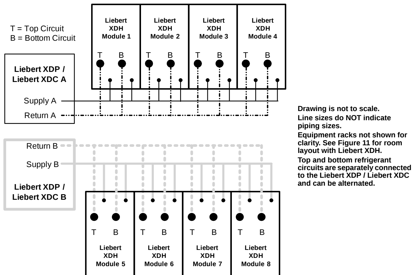
Figure 14 Typical Liebert XDH piping—non-interlaced connection
