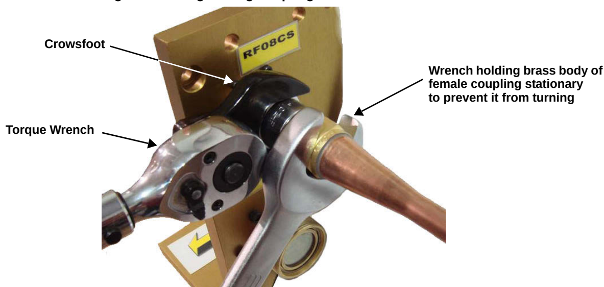
Figure 29 Detail view of Liebert XD Flex Pipe and prefabricated piping port
