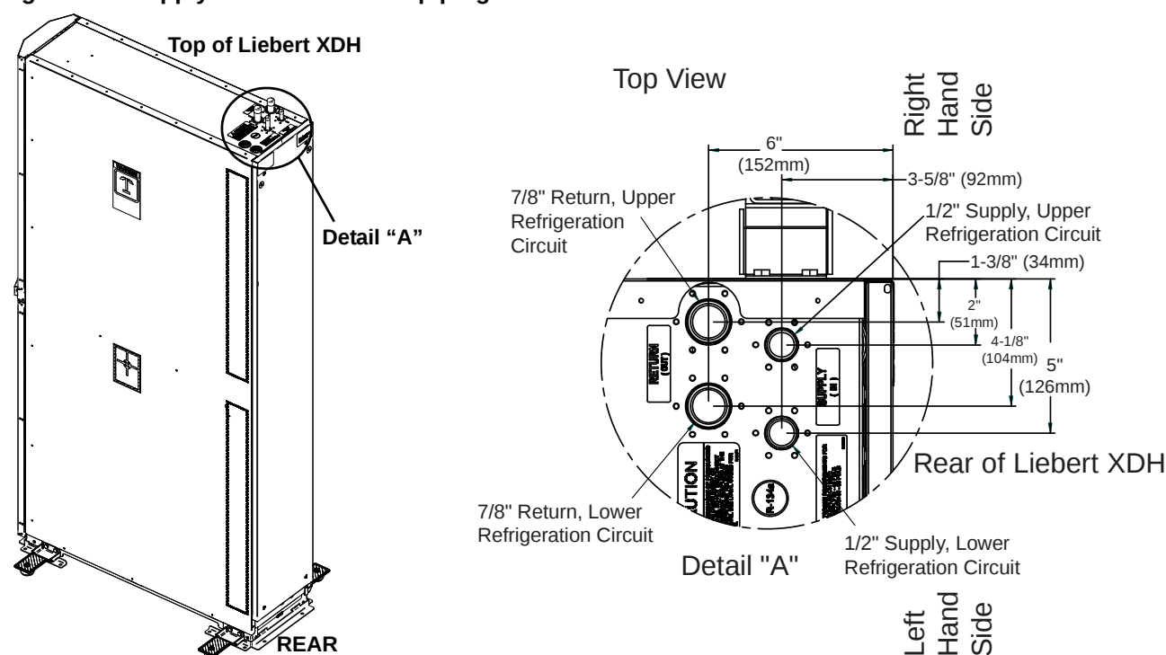
Figure 15 Supply and return—hard-piping connections
