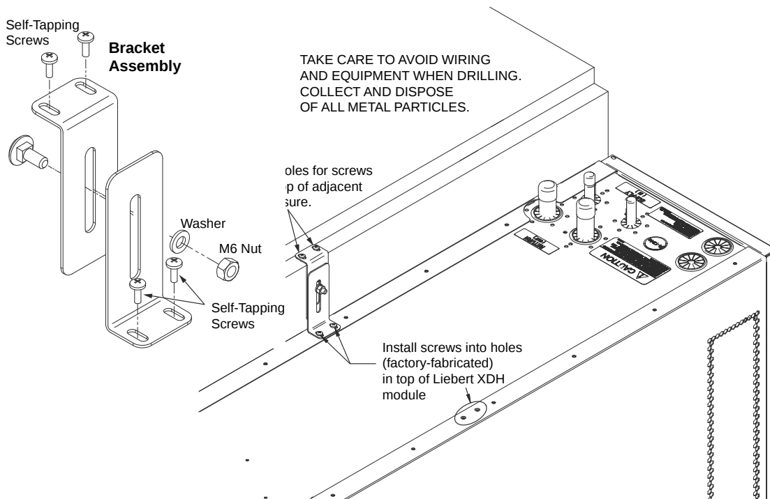
Figure 10 Install tie-down bracket
