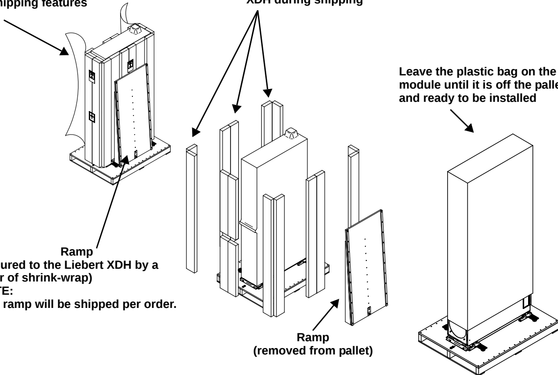
Figure 5 Removing domestic shipping packaging
