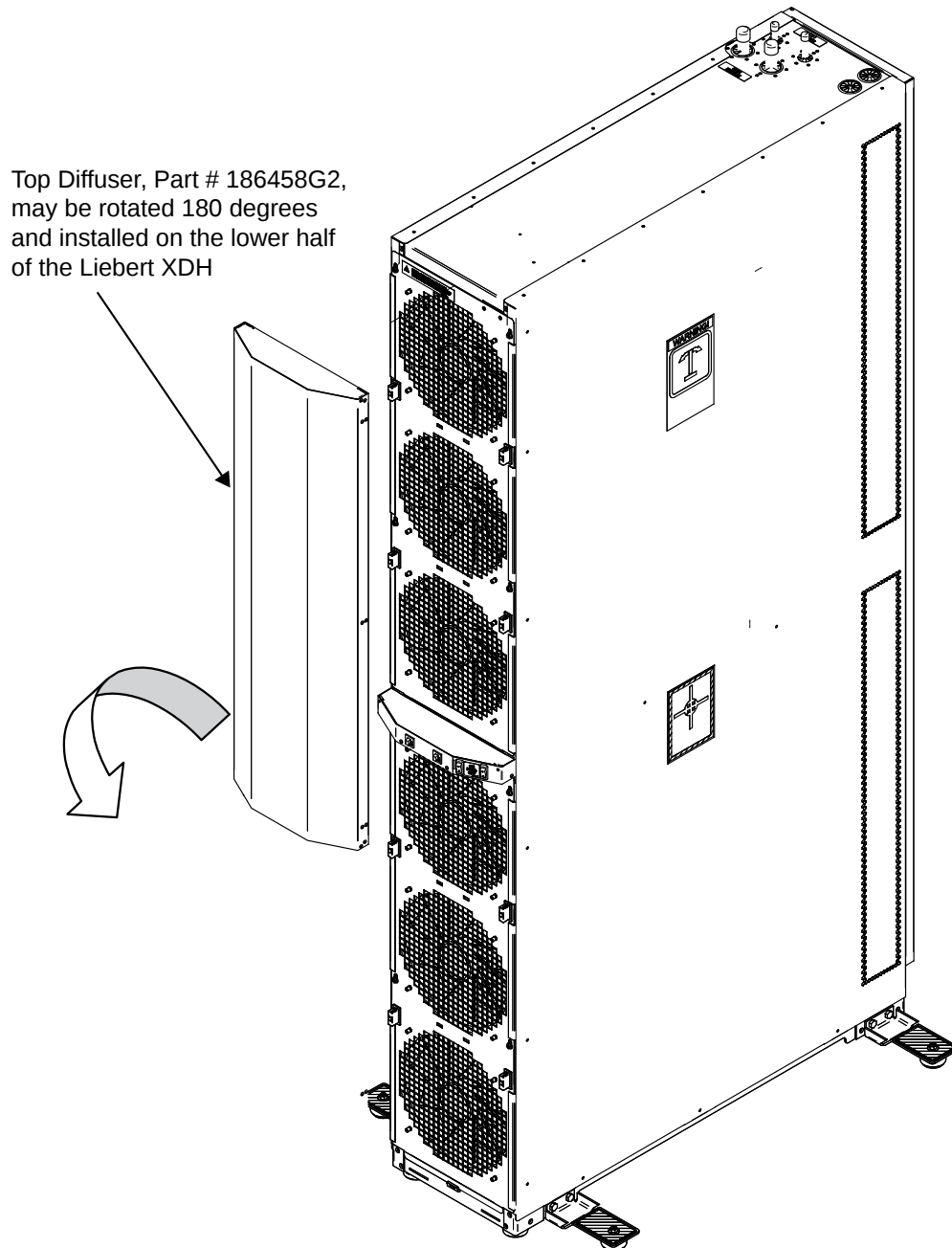
Figure 12 Change airflow direction
