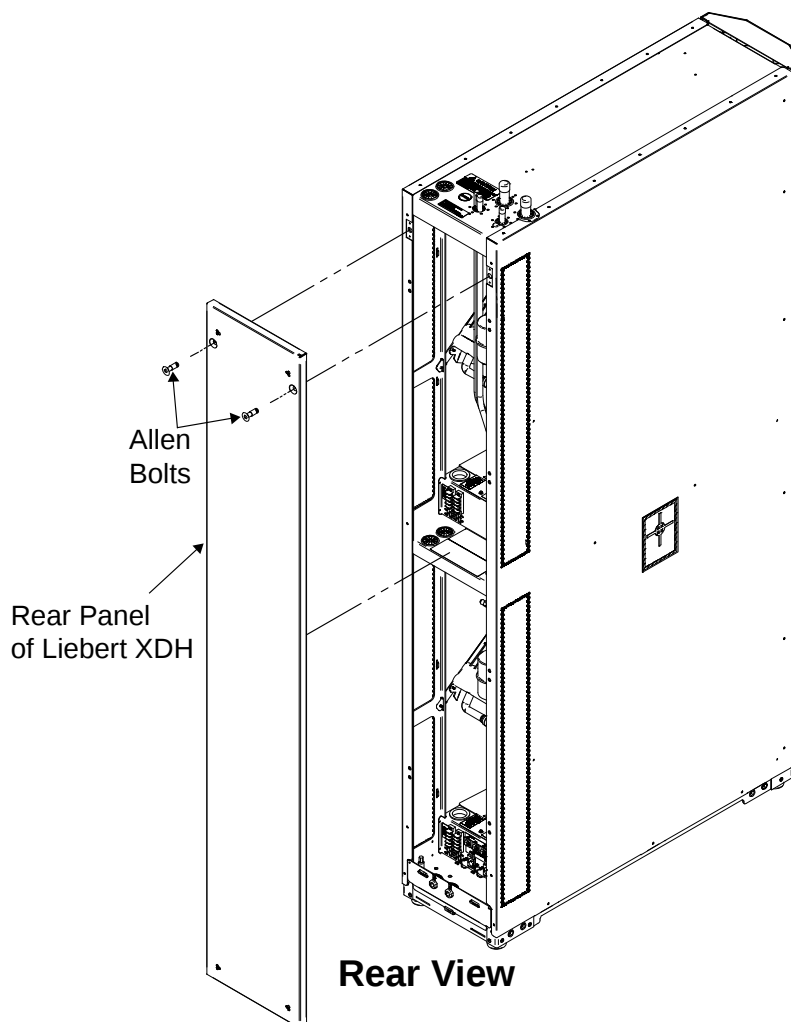
Figure 52 Remove Liebert XDH rear panel
