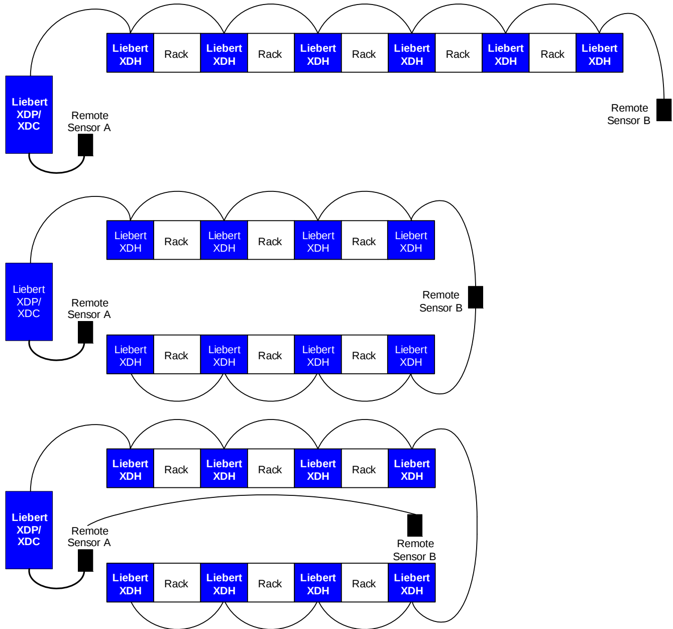
Figure 38 Modules on a single chain
