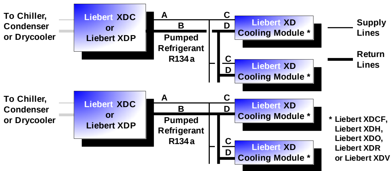
Figure 16 Generic piping layout
