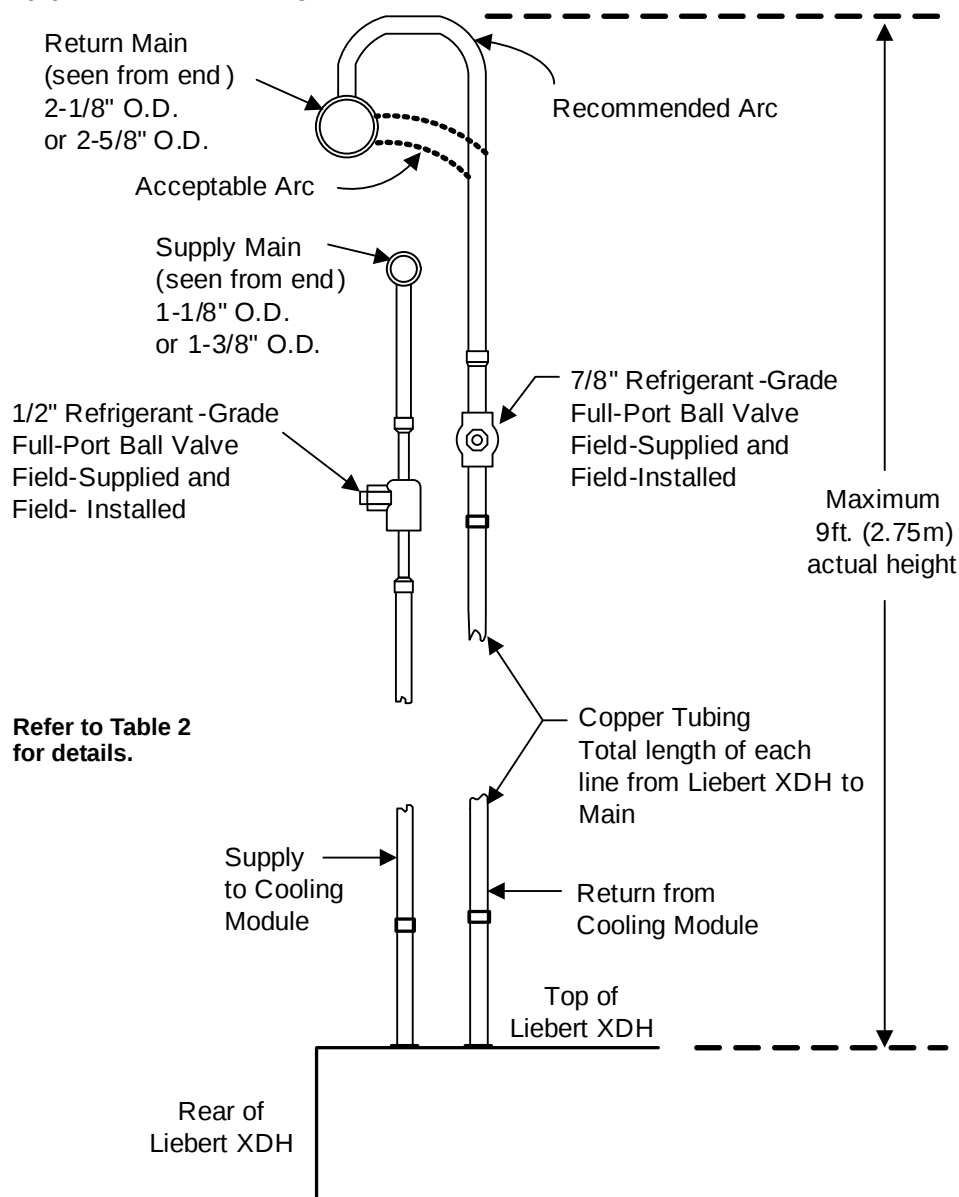
Figure 17 Hard-piped connection diagram
