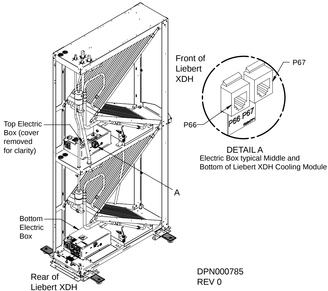
Figure 44 Liebert XDH CANbus port locations
