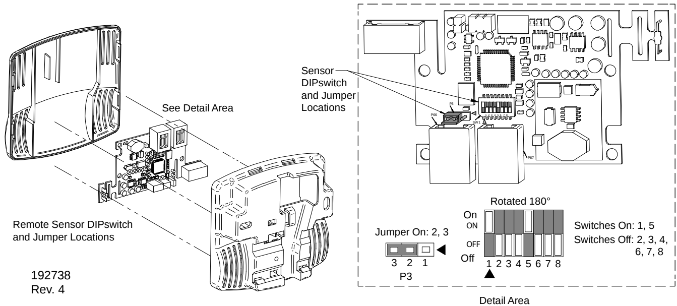
Figure 47 Removing the remote sensor cover
