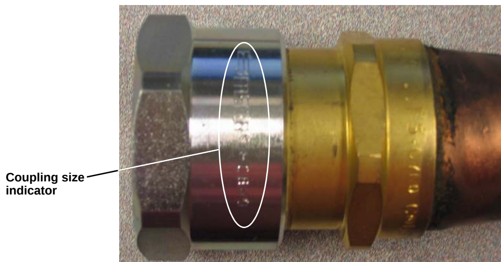
Figure 25 Coupling size indicator
