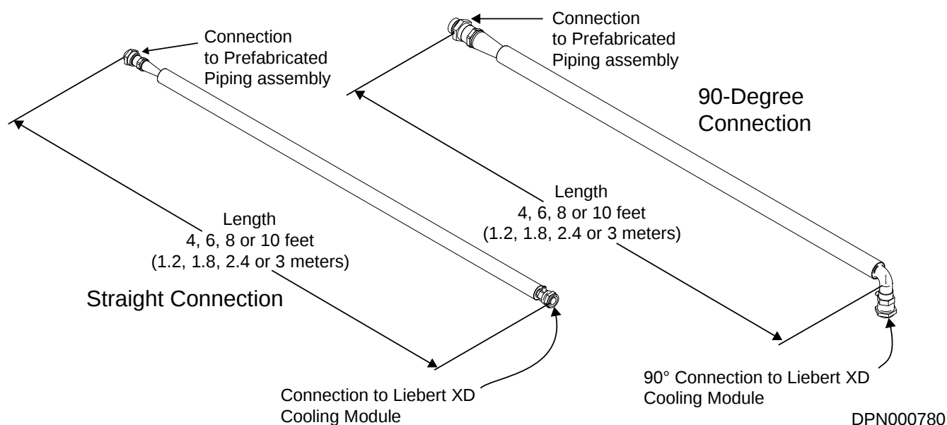
Figure 18 Liebert XD Flex Pipe dimensions—straight and 90-degree connections
