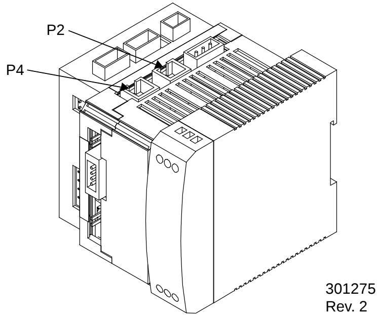
Figure 43 P2 and P4 locations on the CAN isolator
