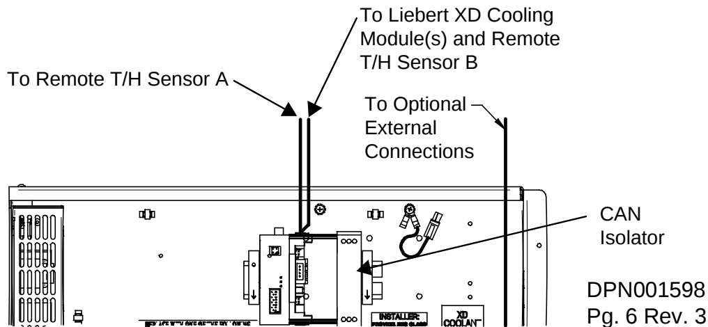
Figure 42 CAN isolator location in the Liebert XDP/XDC
