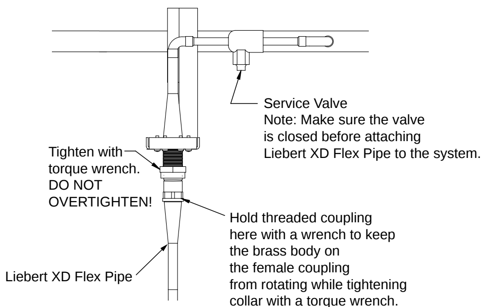
Figure 29 Detail view of Liebert XD Flex Pipe and prefabricated piping port
