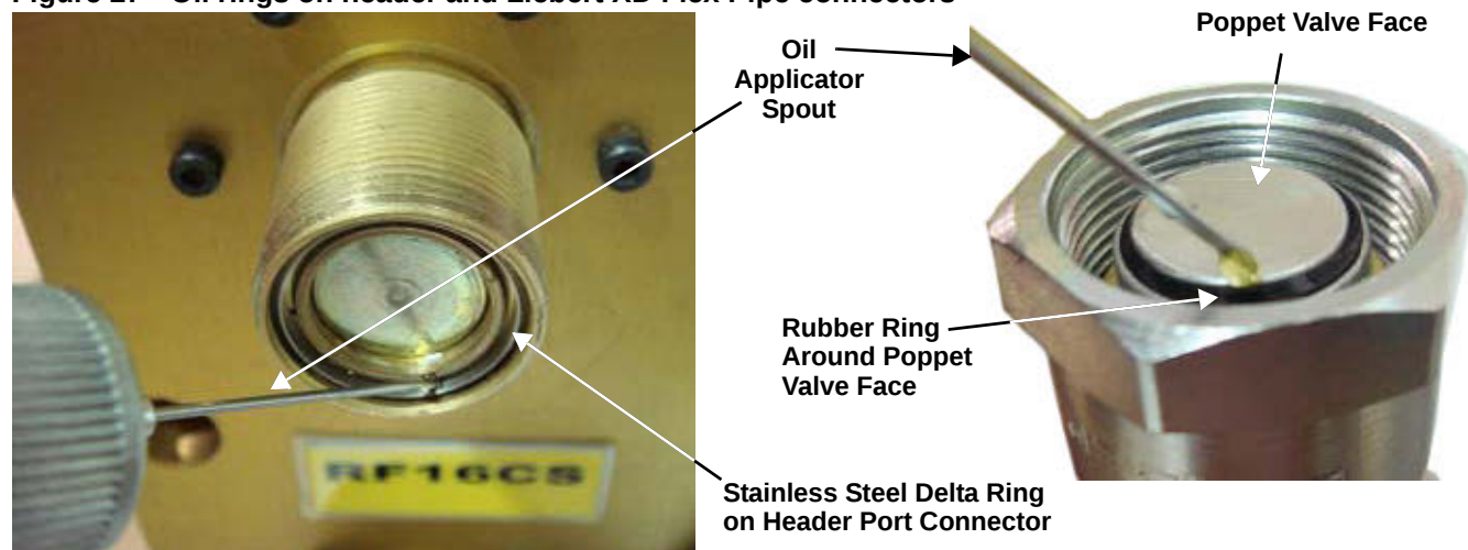
Figure 27 Oil rings on header and Liebert XD Flex Pipe connectors
