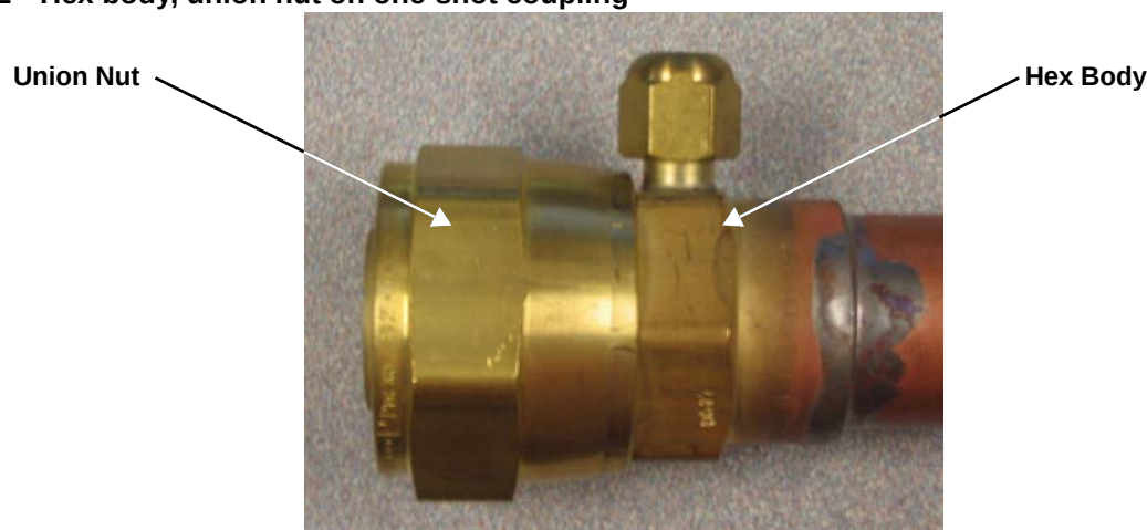
Figure 22 Hex body, union nut on one-shot coupling
