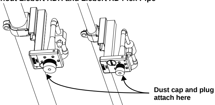
Figure 32 Piping mains without Liebert XDH and Liebert XD Flex Pipe
