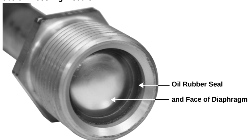
Figure 20 Male coupling on Liebert XD cooling module
