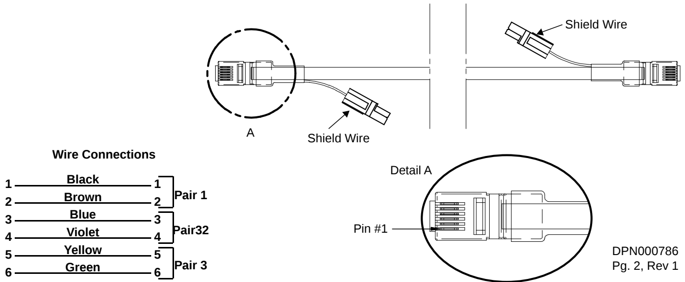
Figure 41 CANbus cable plug
