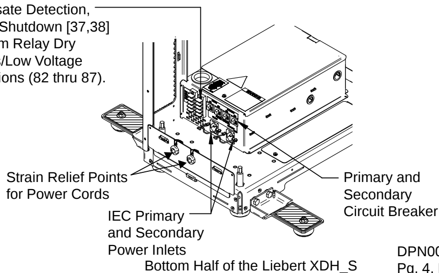
Figure 35 Smart Liebert XDH electrical connections
