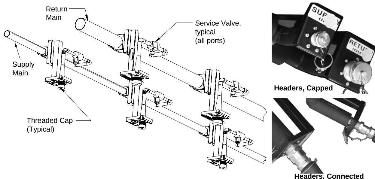
Figure 26 Liebert XD prefabricated piping assembly
