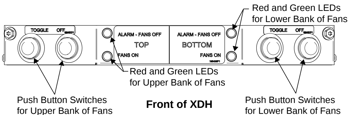
Figure 50 Fan switches, Liebert XDH smart modules
