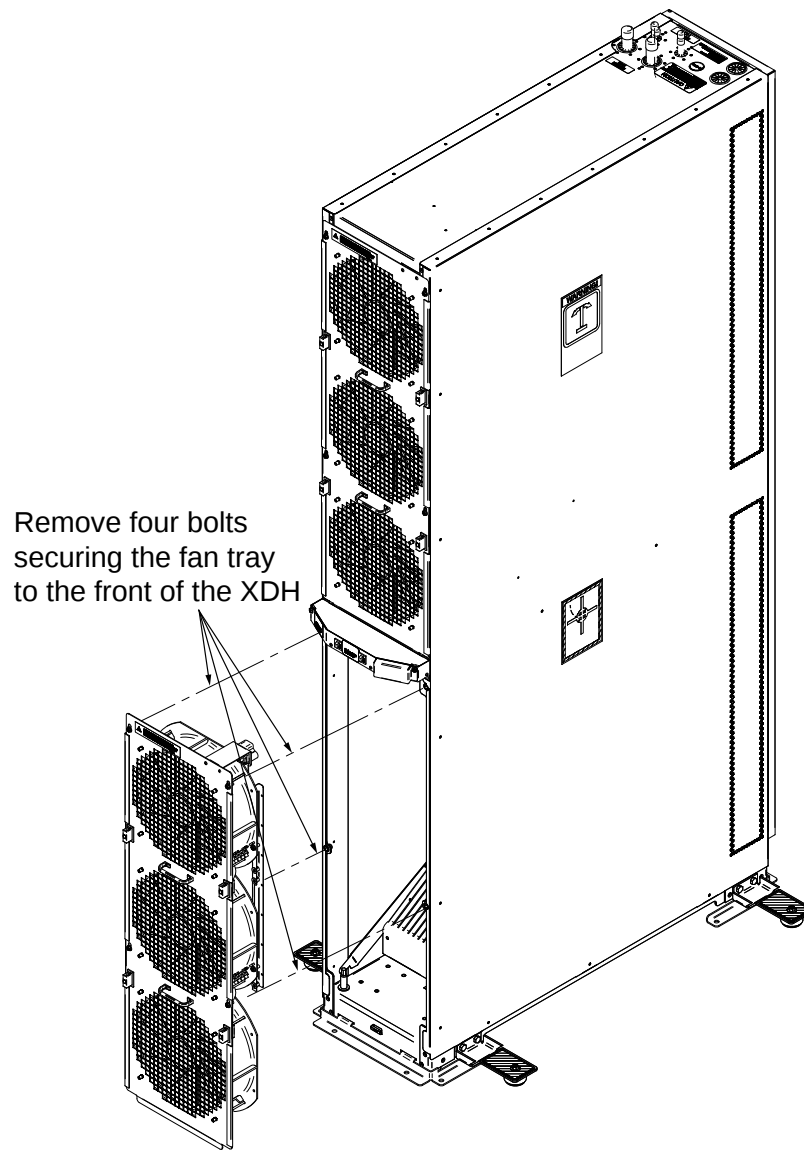
Figure 51 Removing the fan tray
