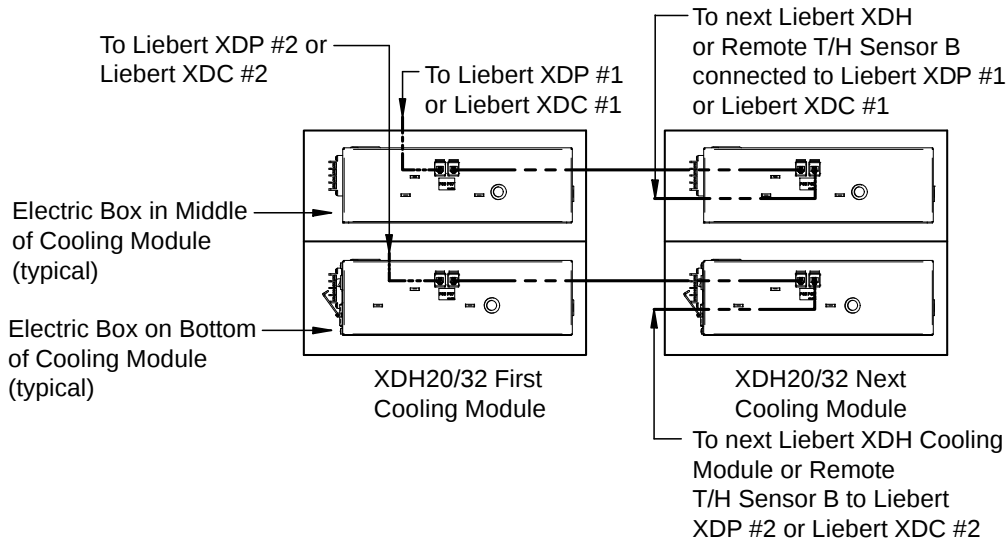
Figure 46 Dual-circuited Liebert XDHs
