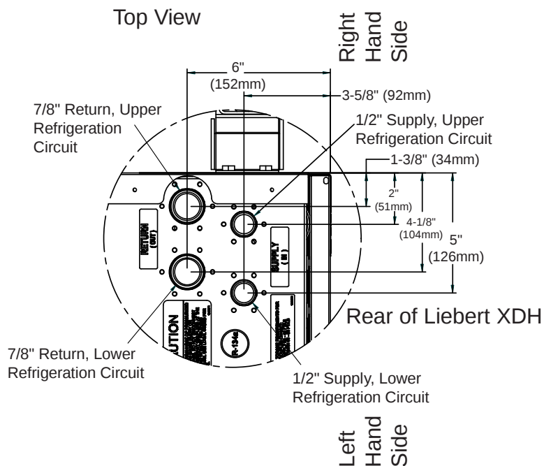
Figure 23 Piping location and connecting sizes for pre-charged modules
