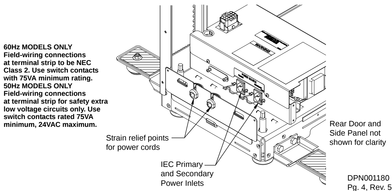
Figure 35 Smart Liebert XDH electrical connections
