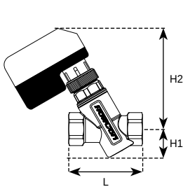
Valve model: A DN15/20/25 with FB actuator
