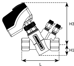
Valve model: AB DN15/20/25 with FM.0 actuator
