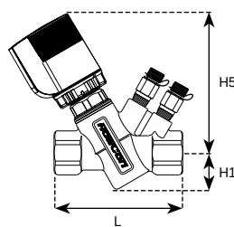
Valve model: AB DN15/20/25 with FT actuator
