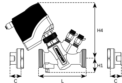
Valve model: ABV1 DN15/20/25 with FM.1 actuator
