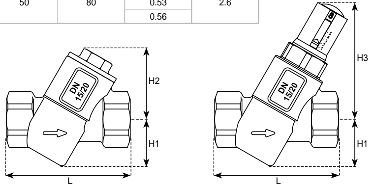
FlowCon A with composite cartridge
