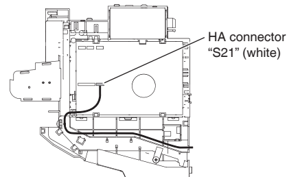
How to route the HA connection cord
