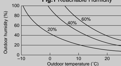
Fig.1 Reachable Humidity
