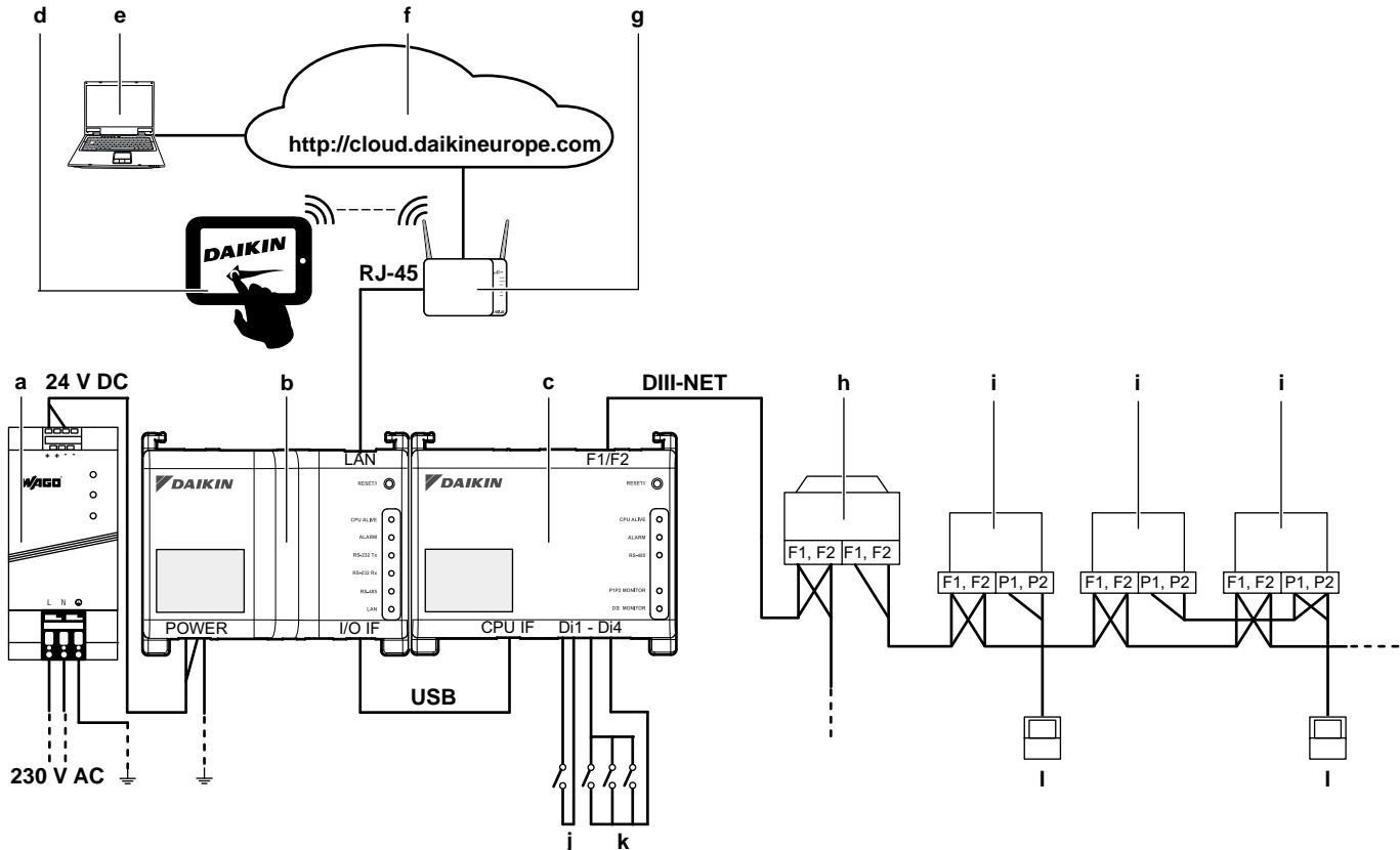
Schematic setup of the intelligent Tab Controller
