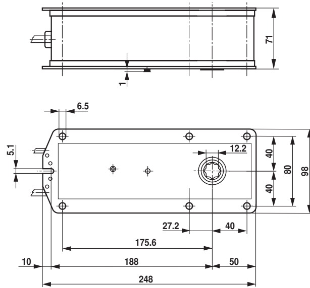
Dimensional diagrams
