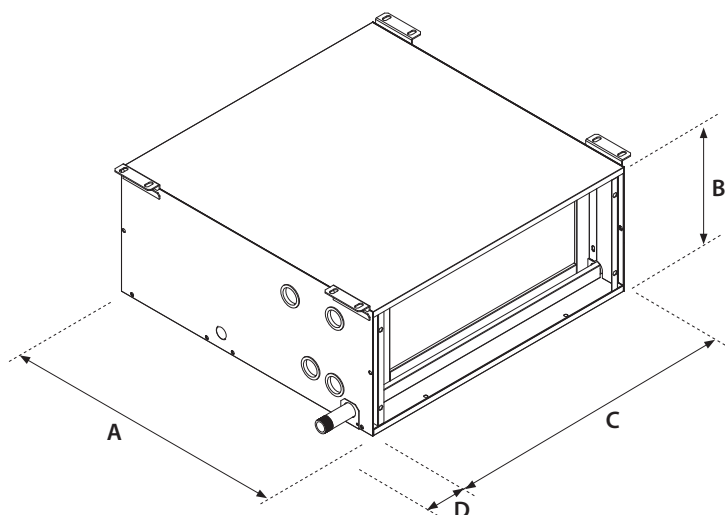
TA HORIZONTAL INSTALLATION AND WITH EXTRACTOR
