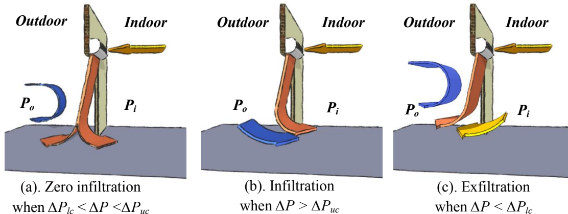
Fig. 1. Infiltration/exfiltration characteristics of an air curtain jet under different pressure differences, \Delta P = P_o - P_i (note that the zero infiltration does not apply to the air recirculating through the air curtain).
