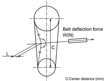
(Figure 2) Belt tension
