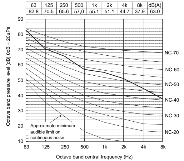
PFD-P500VM-E (External static pressure 120Pa)
