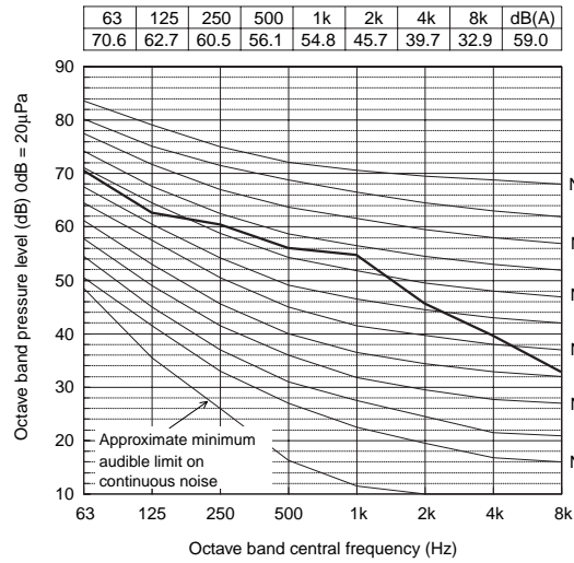
PFD-P250VM-E (External static pressure 120Pa)
