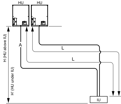
Fig.IV-1-(2)B : PQHY Piping Design
