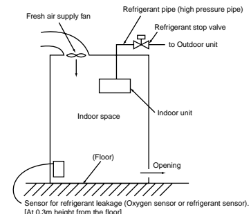
Fig.8-4. Fresh air supply and refrigerant shut-off upon sensor action
