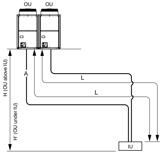
Fig.IV-1-(2)A : PUHY Piping Design
