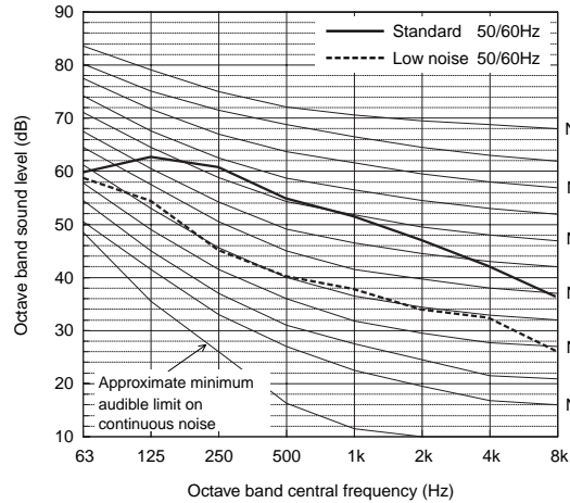
PQHY-P250YHM-A (External static pressure 0Pa)
