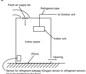
Fig.8-3. Fresh air supply upon sensor action
