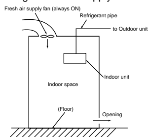
Fig.8-2. Fresh air supply always ON
