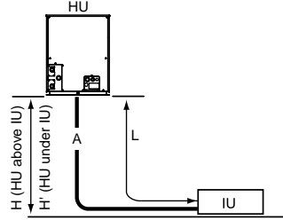
Fig.IV-1-(1)B : PQHY Piping Design
