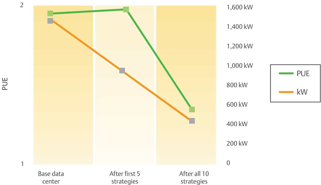
Figure 14. The first five strategies in Energy Logic 2.0 produce a dramatic reduction in energy consumption but a small increase in PUE.
