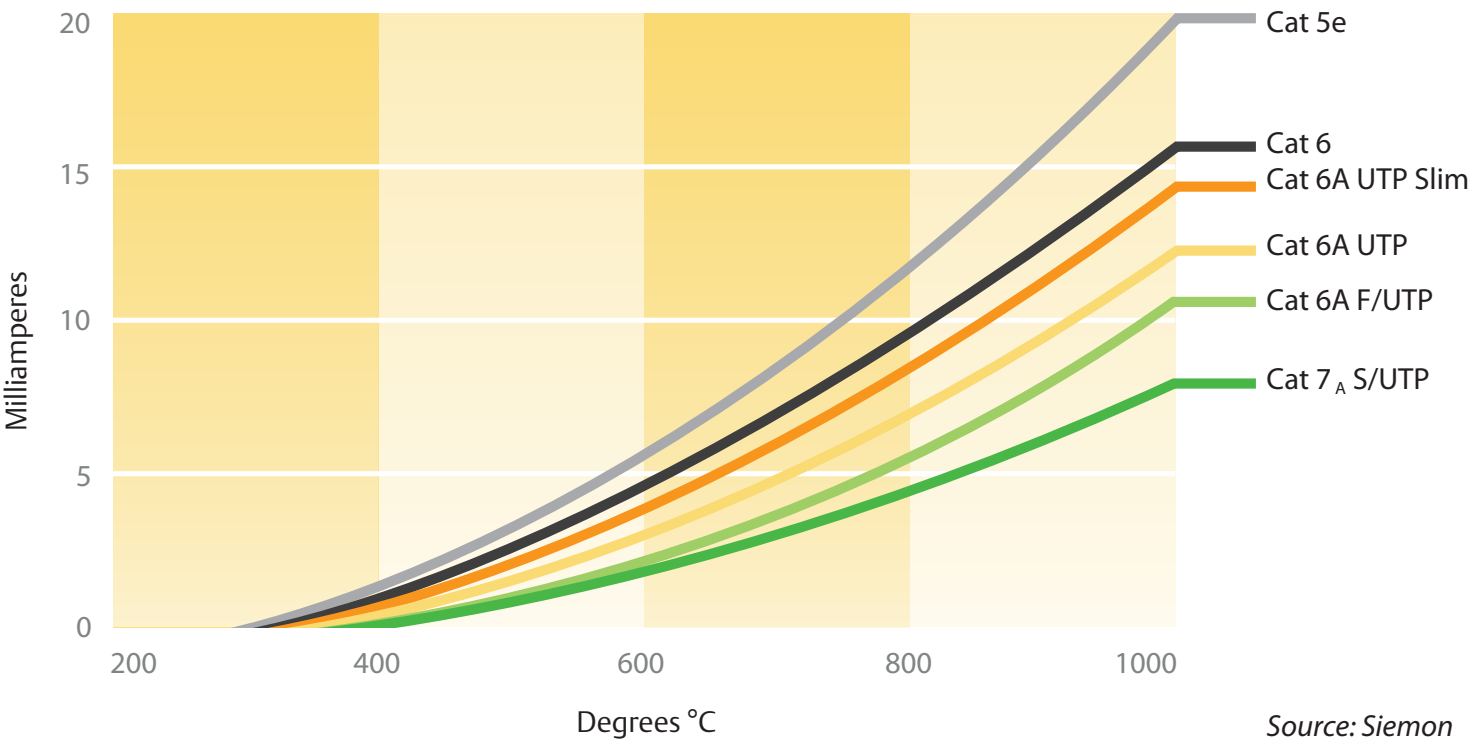
Figure 9. Older communication cables generate more heat, reducing data center efficiency.
