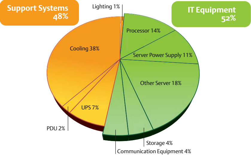
Figure 1. IT systems account for 52 percent of energy consumption in a typical 5,000 square foot (464.5 square meter) data center.
